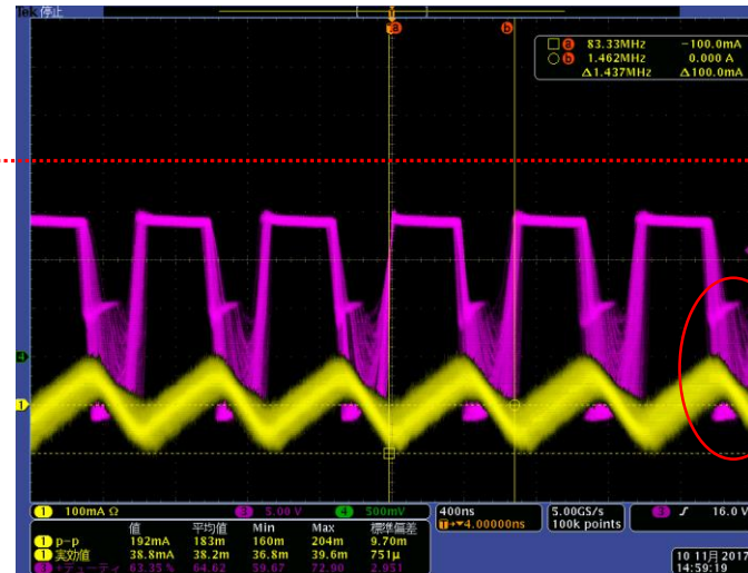
Iout=38mA condition
