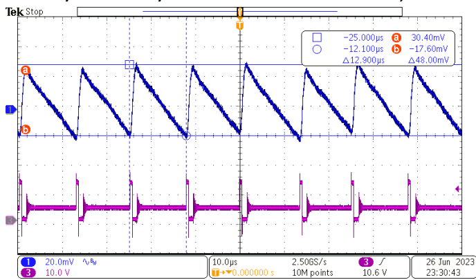
12Vin/3.9Vout/100mA: Channel1:Vout; Channel3:SW
