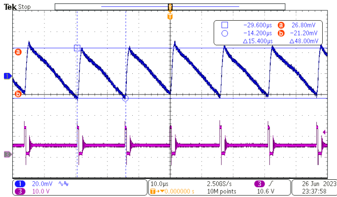
12Vin/3.9Vout/80mA: Channel1:Vout; Channel3:SW
