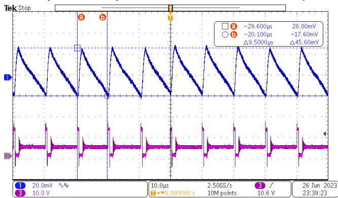
12Vin/3.9Vout/100mA: Channel1:Vout; Channel3:SW
