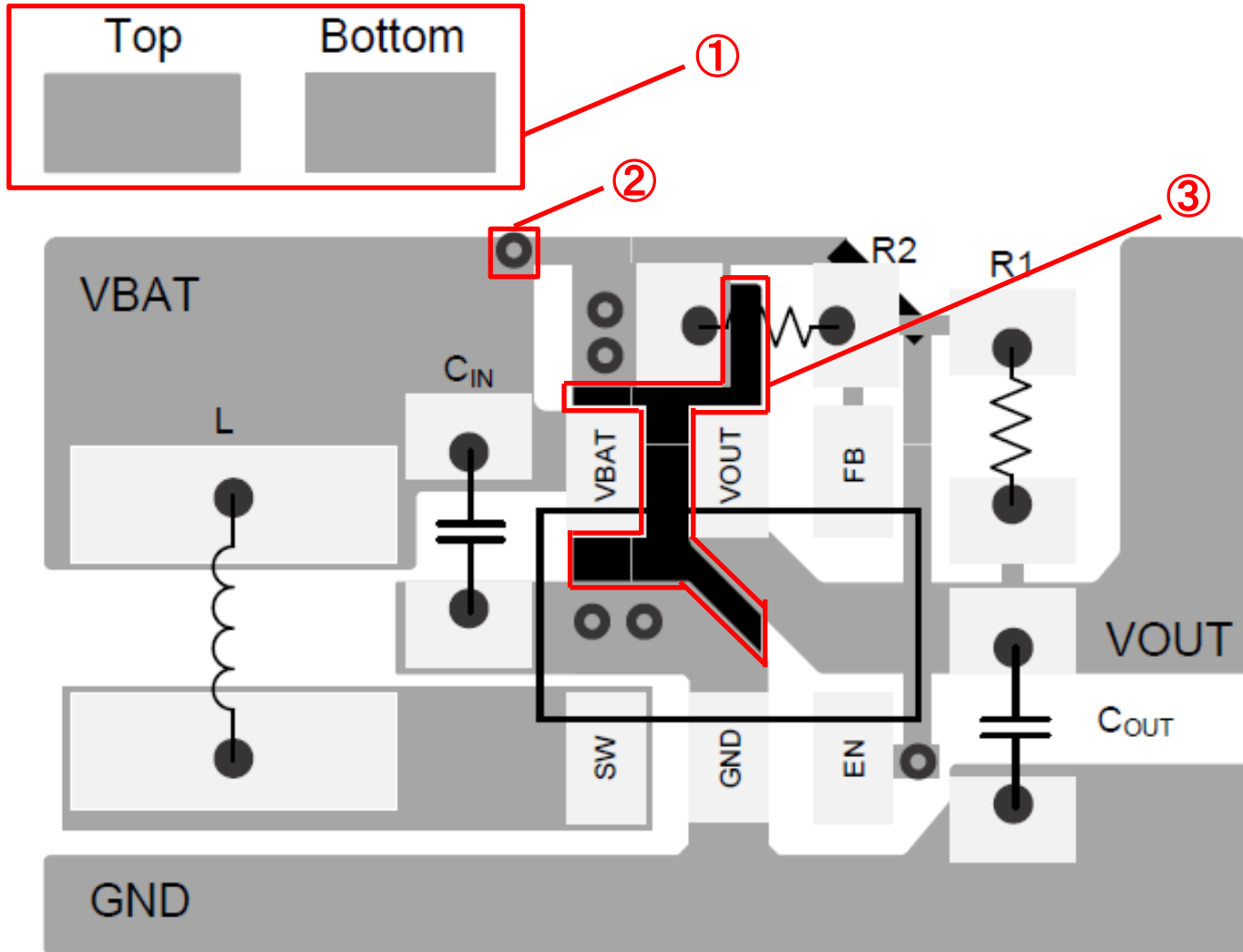
Figure 33. PCB Layout
