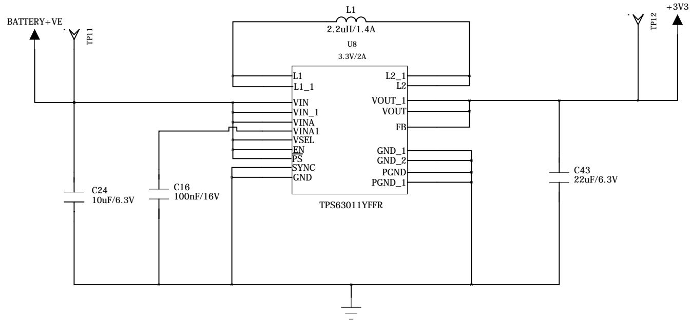
3V3 Buck/Boost Converter
