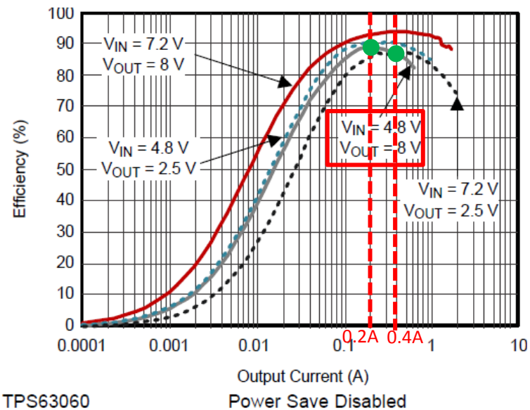
Figure 12. Efficiency vs. Output Current
