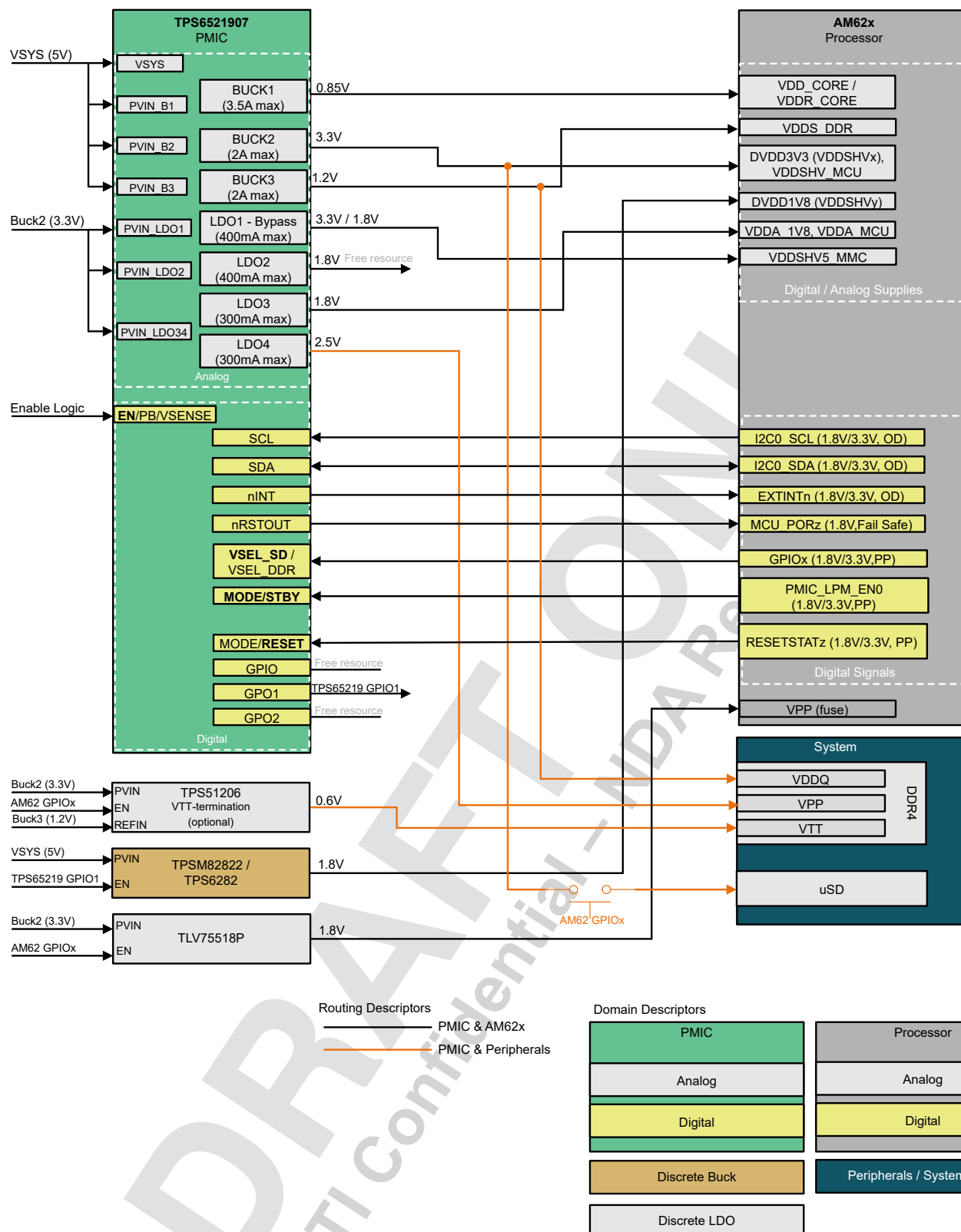
Figure 2-3. TPS6521907 Example Power Block Diagram
