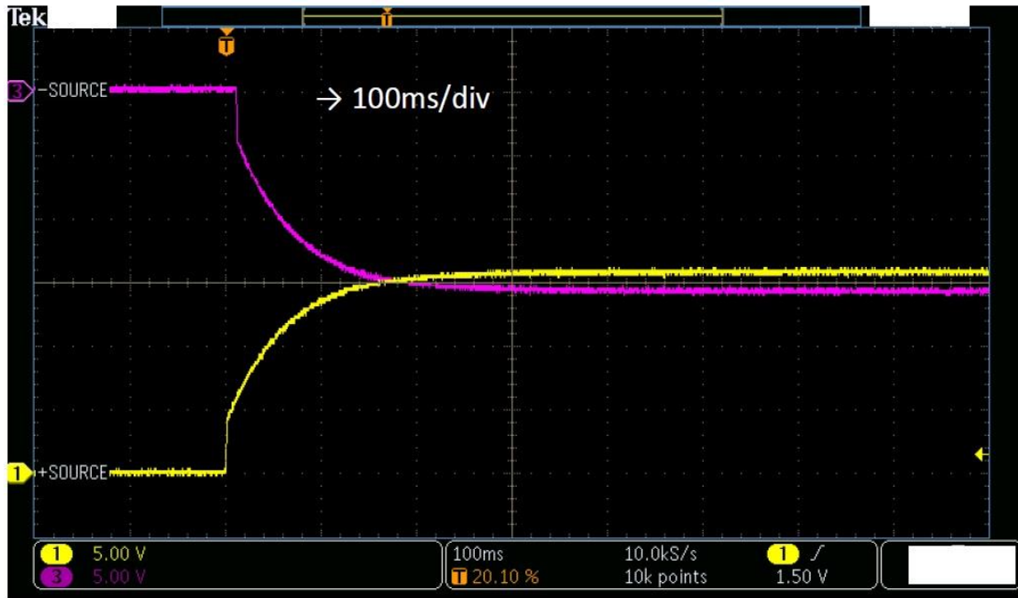
Figure 1 Normal Inp and Inn waveform
