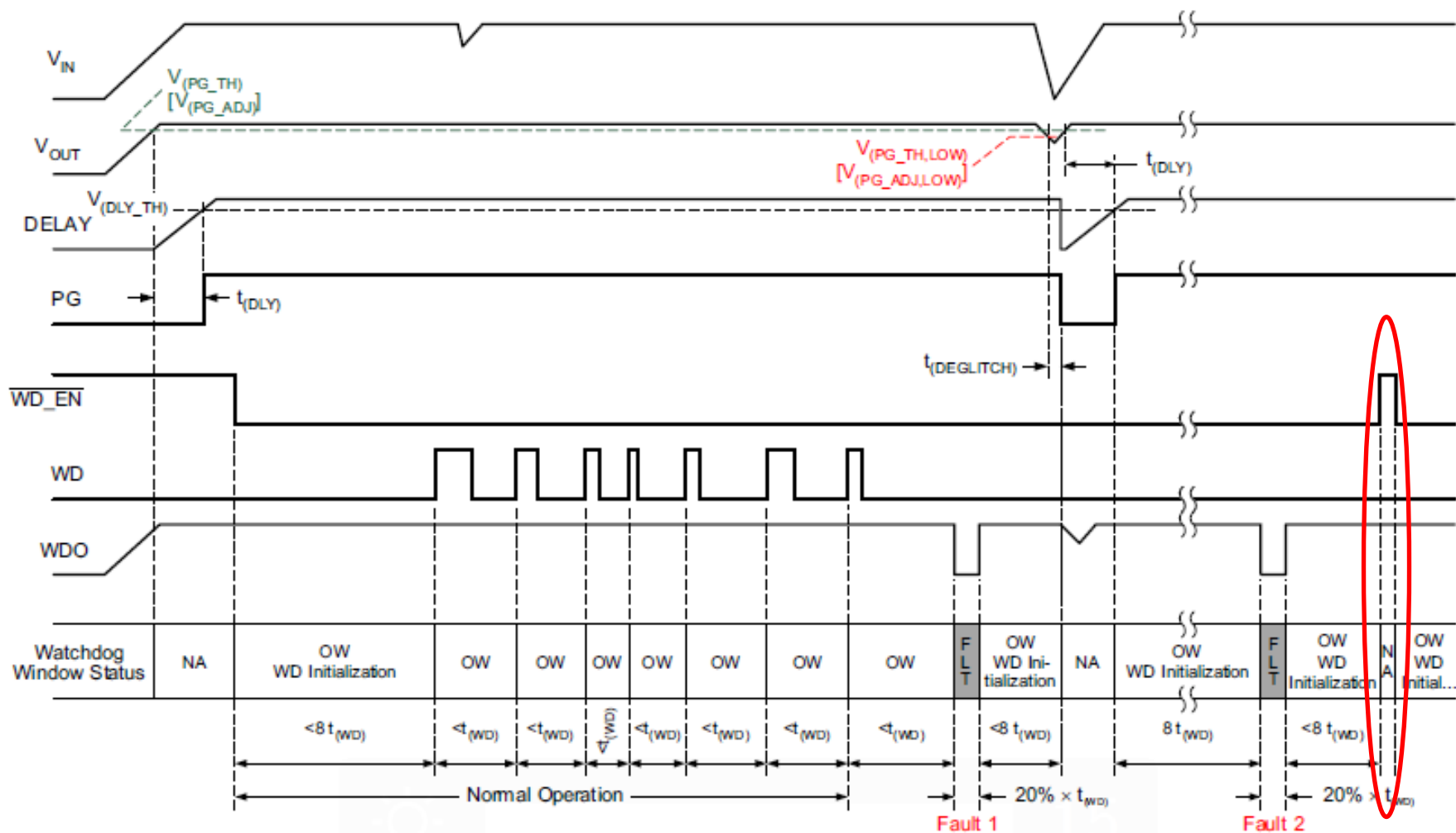
Figure 25. Standard Watchdog Operation
