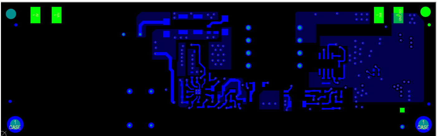
Figure 6: Bottom Layer
