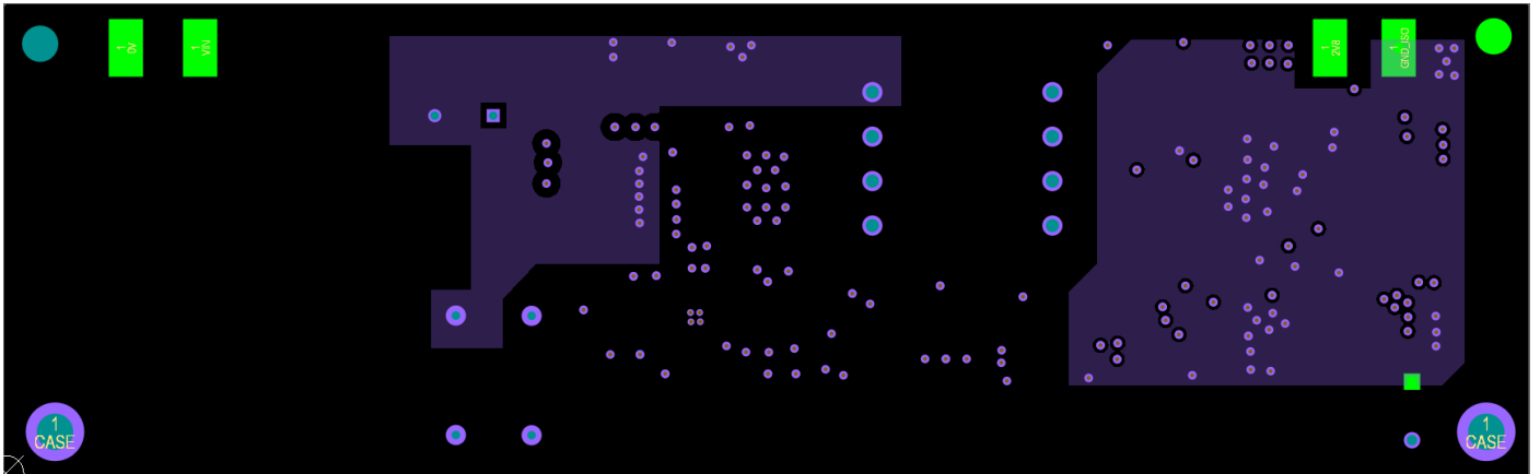
Figure 5: Layer 5
