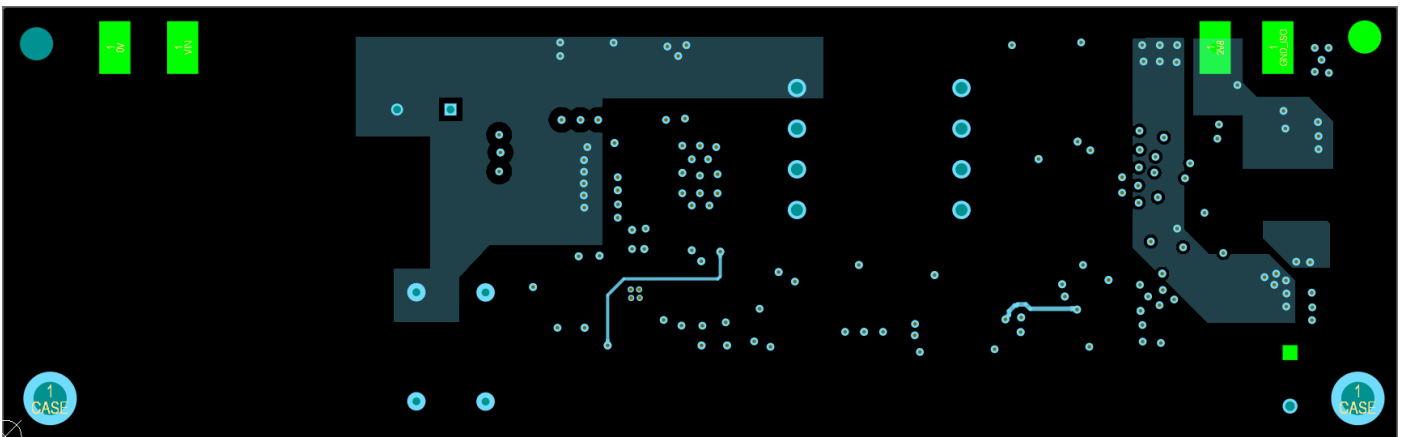
Figure 3: Layer 3
