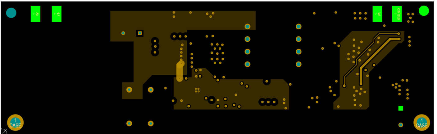
Figure 2: Layer 2
