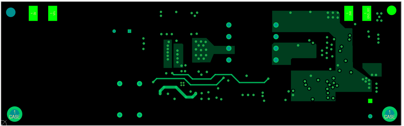
Figure 4: Layer 4
