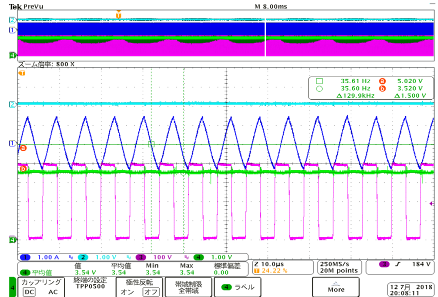
Soft start capacitor series resistance : 330Ω
