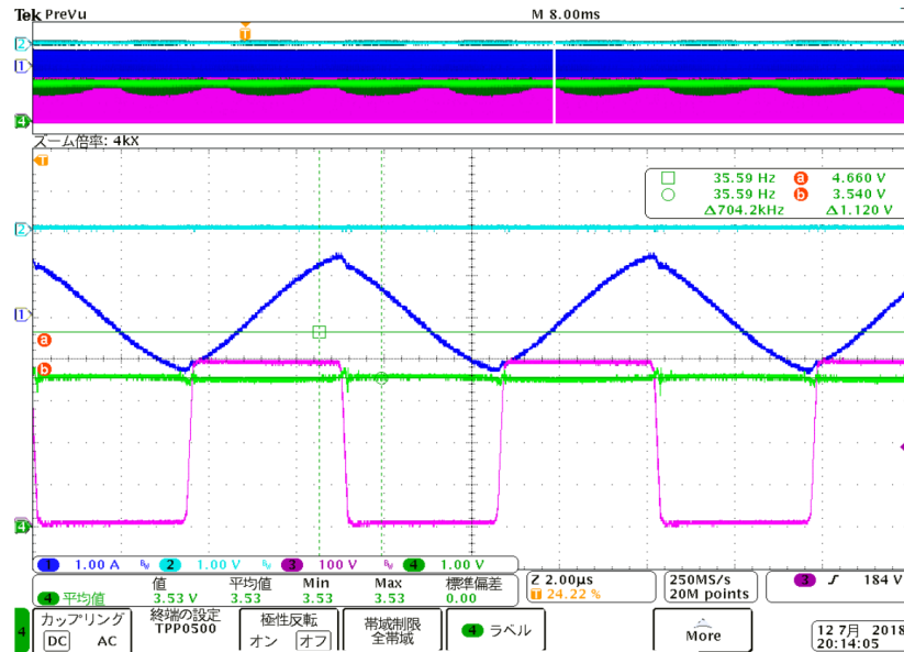
Soft start capacitor series resistance : 100Ω
