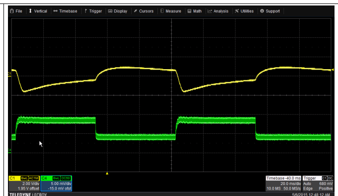
Figure 9. V_{IN} = 265 V_{RMS}
