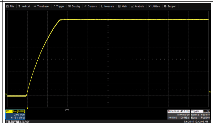
Figure 7. V_{IN} = 265 V , I_{OUT} = 225 mA
