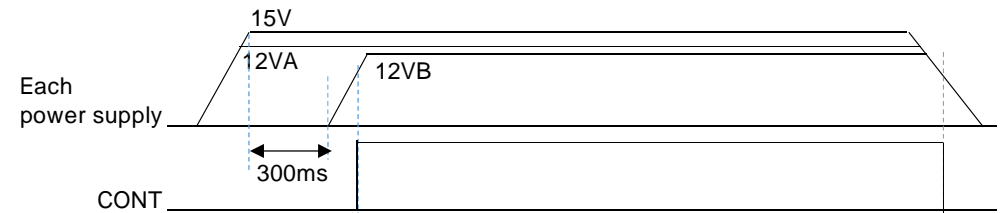
( Power sequence )
