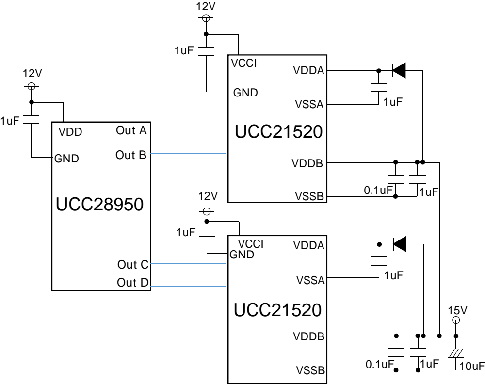
Connection between UCC28950 and UCC21520 and power supply sequence (plan 1)
