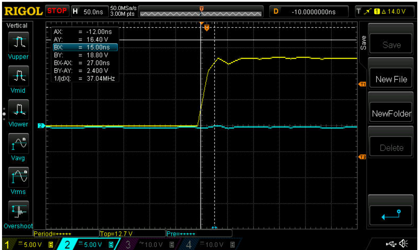
FIGURE 6 - 24mar20 2350 PIN22 OUTA - PIN21 OUTB SIGNALS
