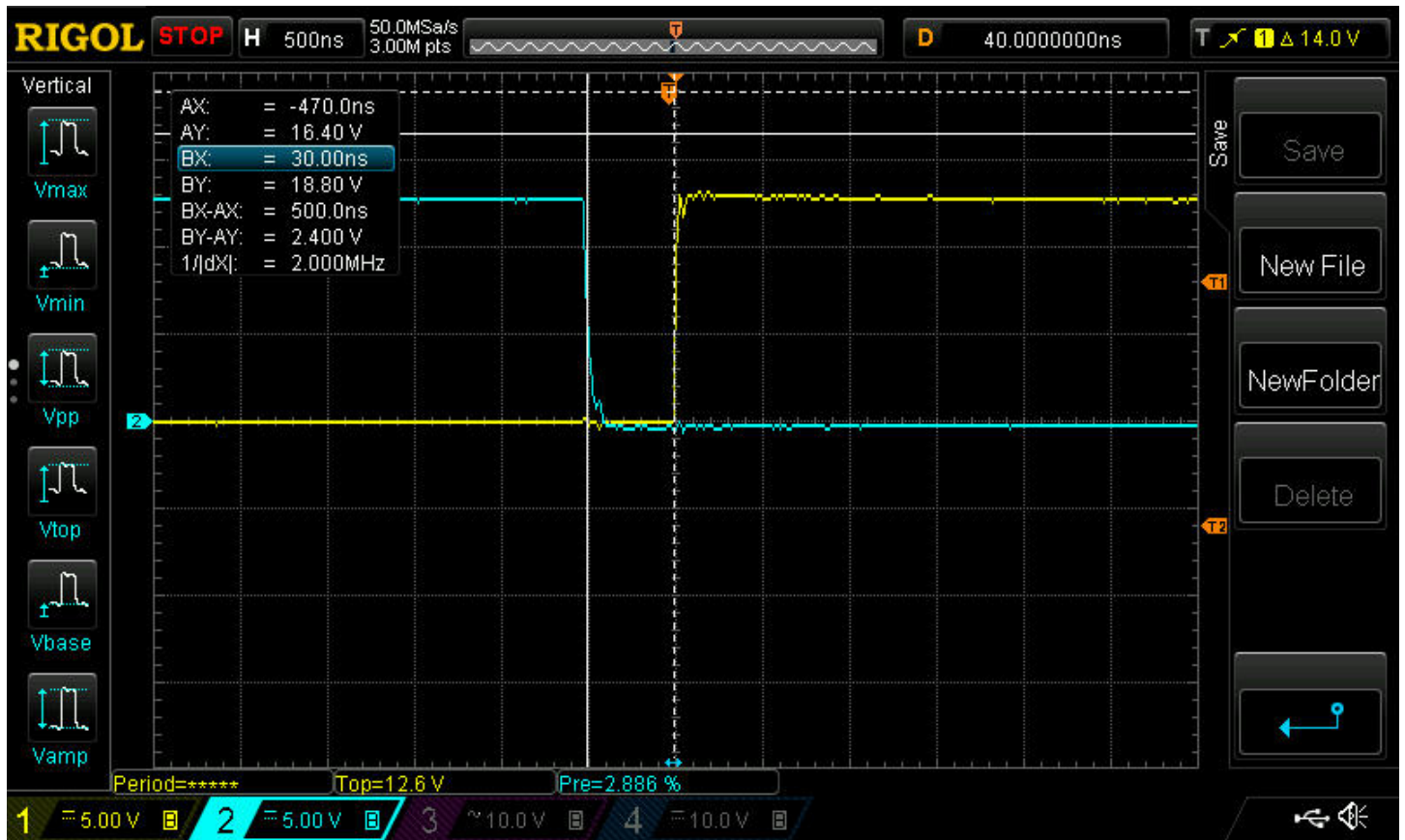
FIGURE 4 - 24mar20 2350 PIN22 OUTA - PIN21 OUTB SIGNALS
