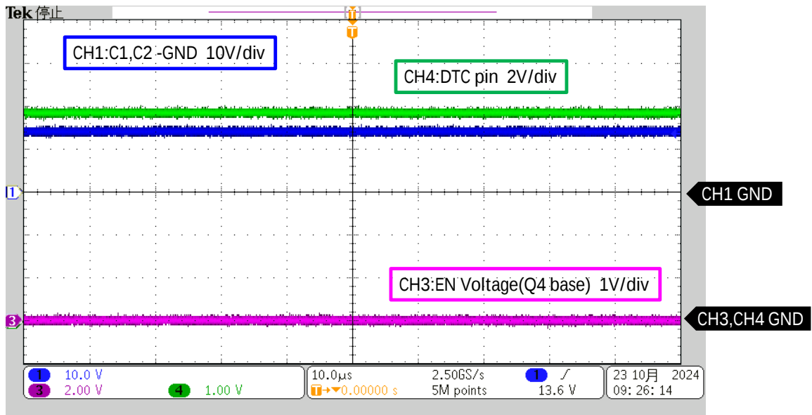
Fig1. ① Before battery recognition EN: Low
