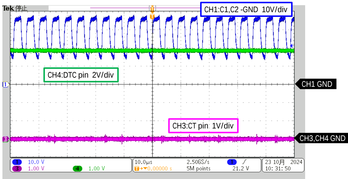
Fig4. Pull down CT to GND
