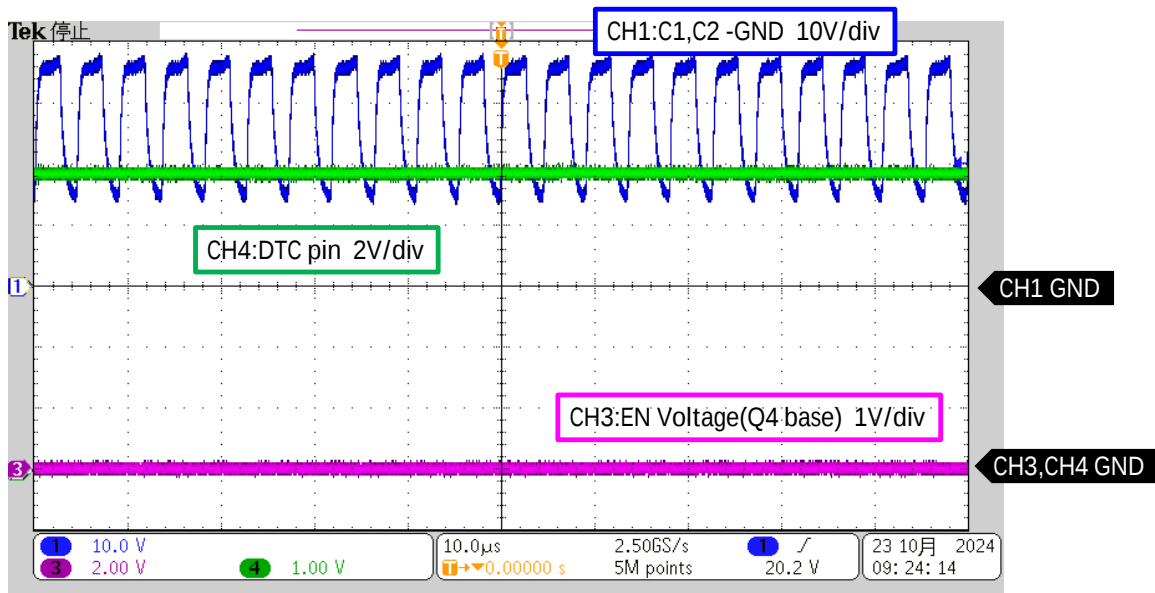
Fig3. ③ When charging ends EN: Low
