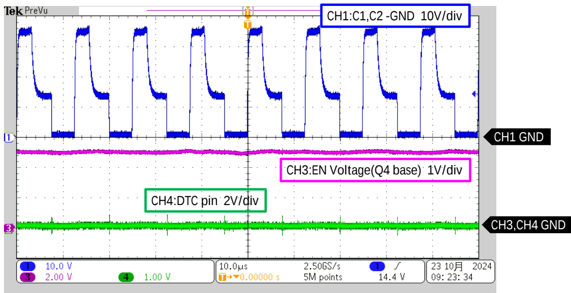
Fig2. ② After battery recognition EN: High
