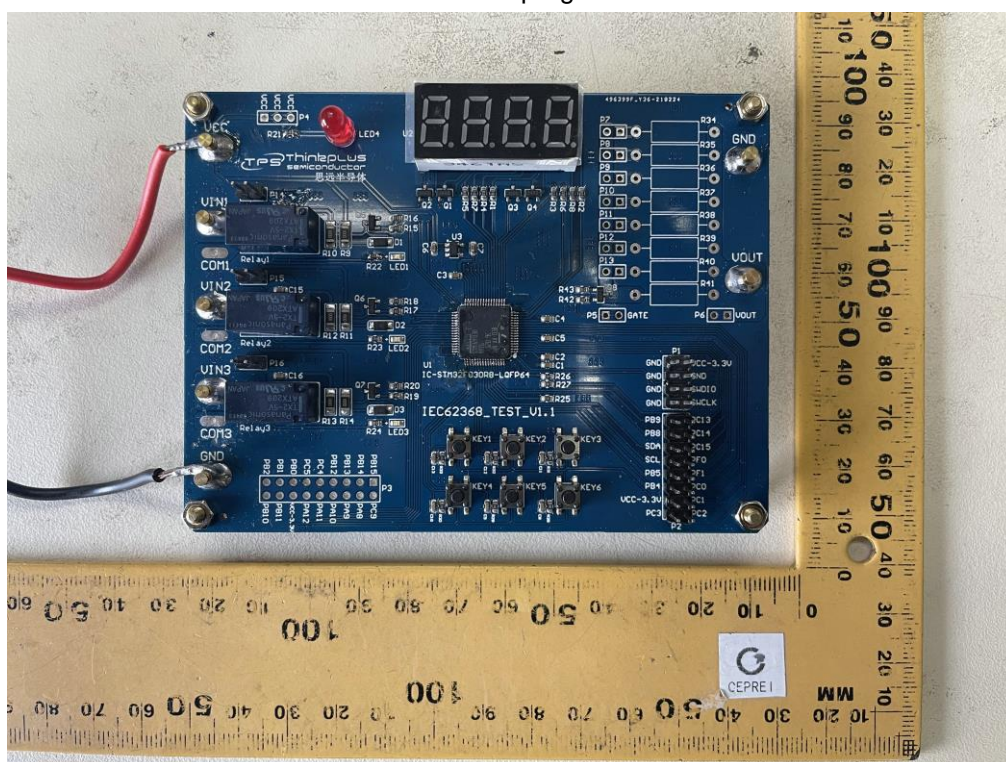
Control circuits for test programs of Annex G
