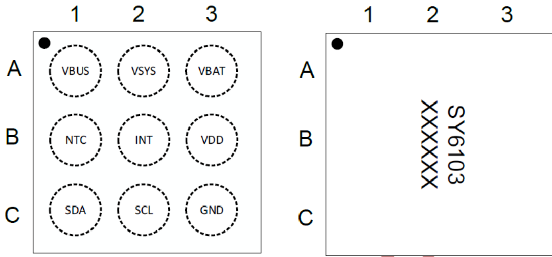
PIN assignment of SY6103
