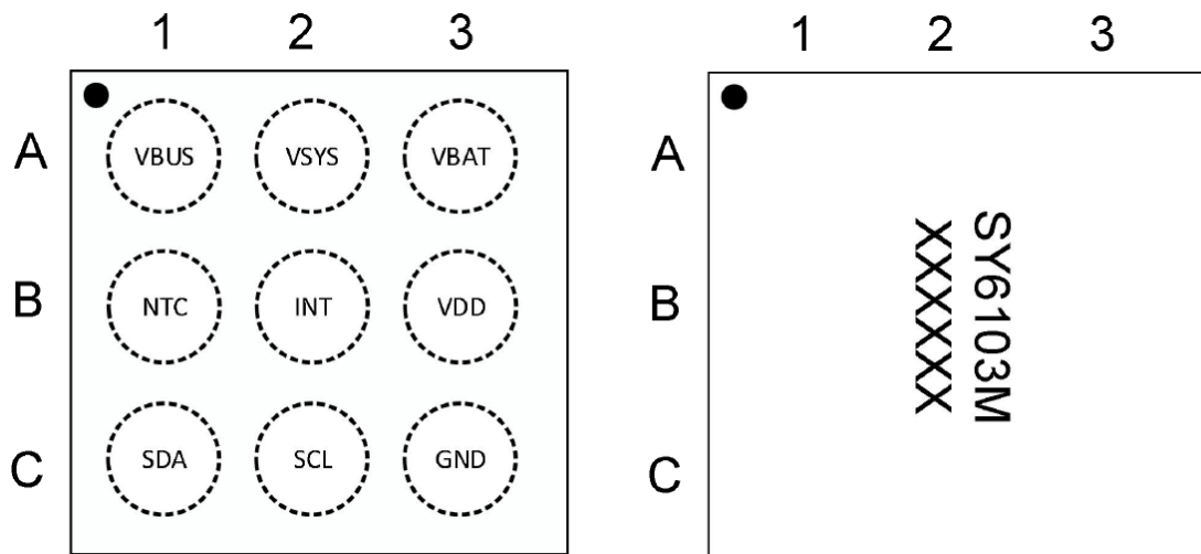
PIN assignment of SY6103M
