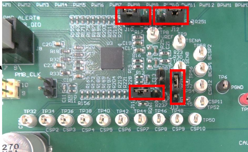
Jumper Position For 10+2
