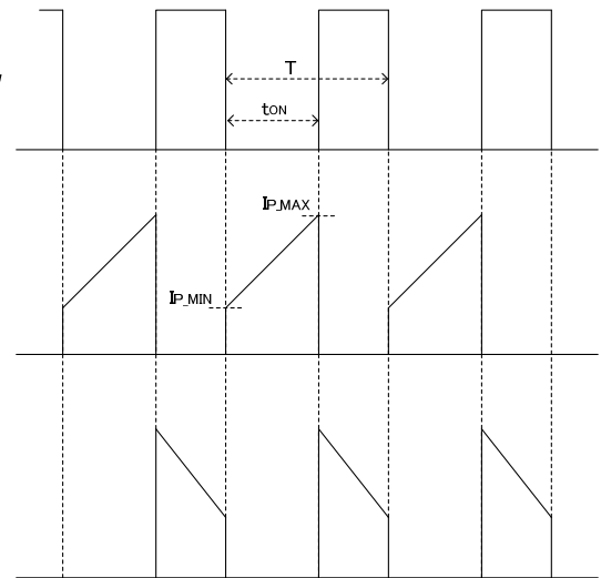
Figure 29. Monitor of the Amount of Load Compensation (Continuous Mode)
