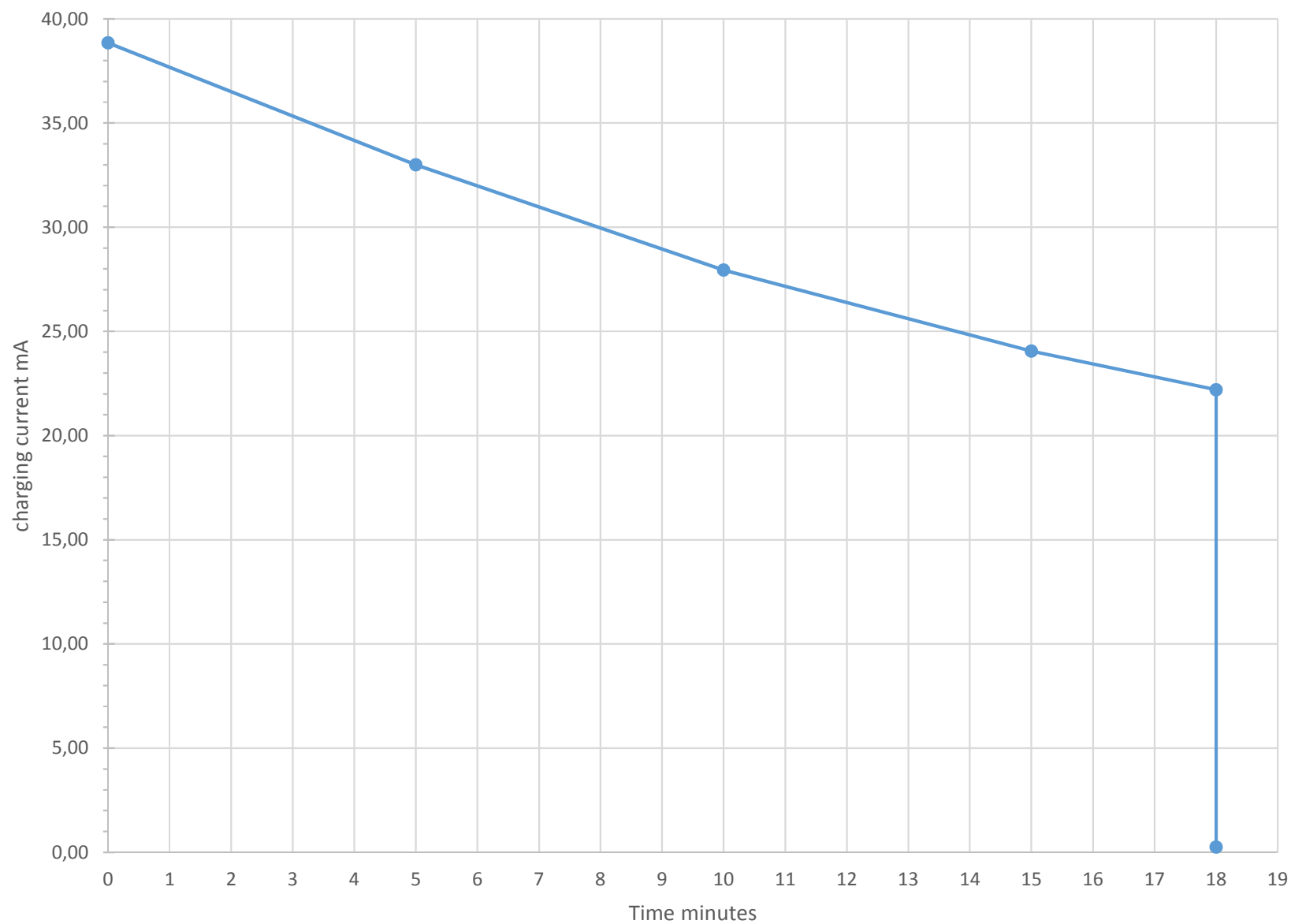
14-07-2017, bq21040 charging current passing termination, Riset = 2k7
