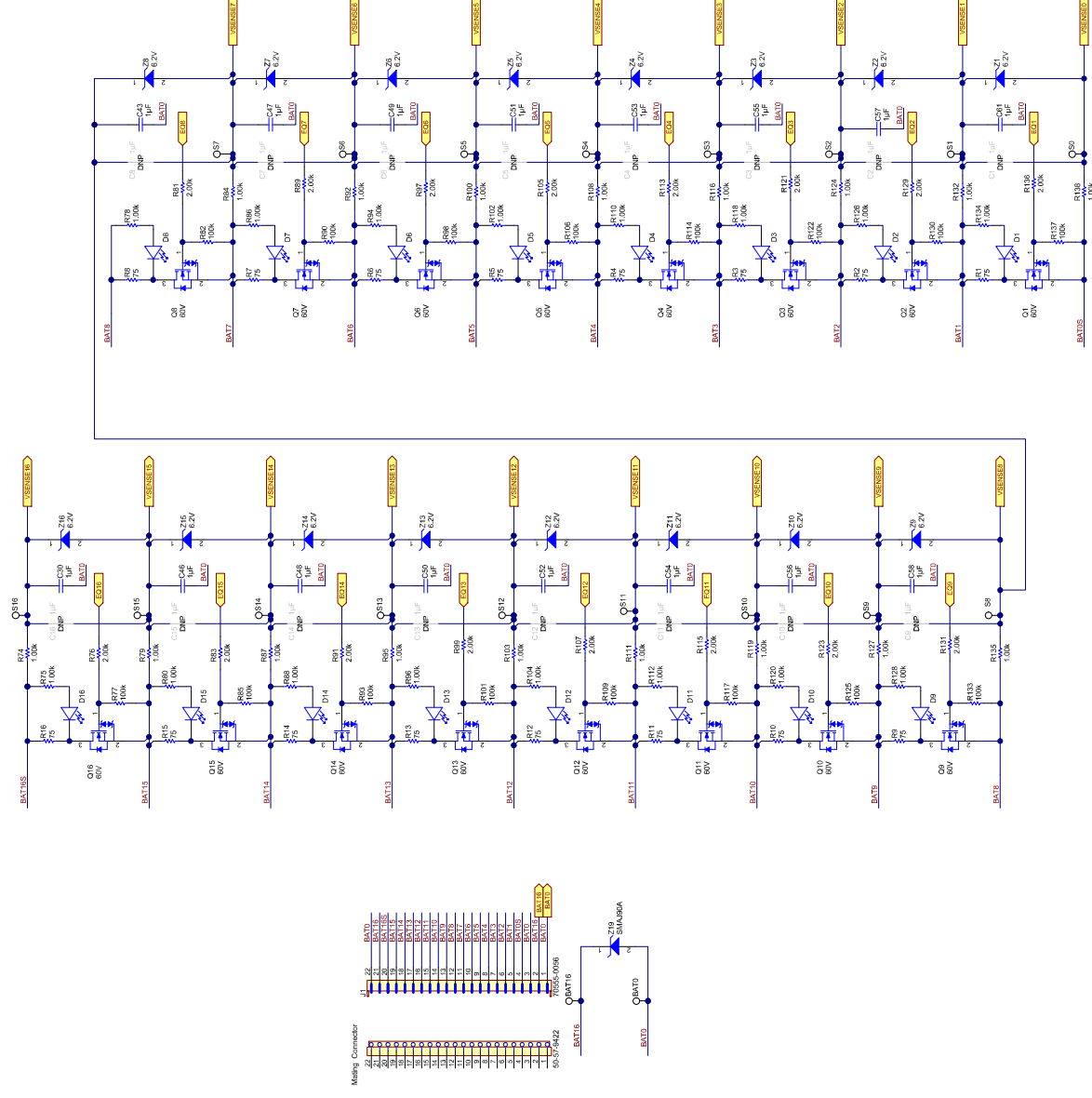
Figure 43. bq76PL455EVM Schematic - Sheet 2
