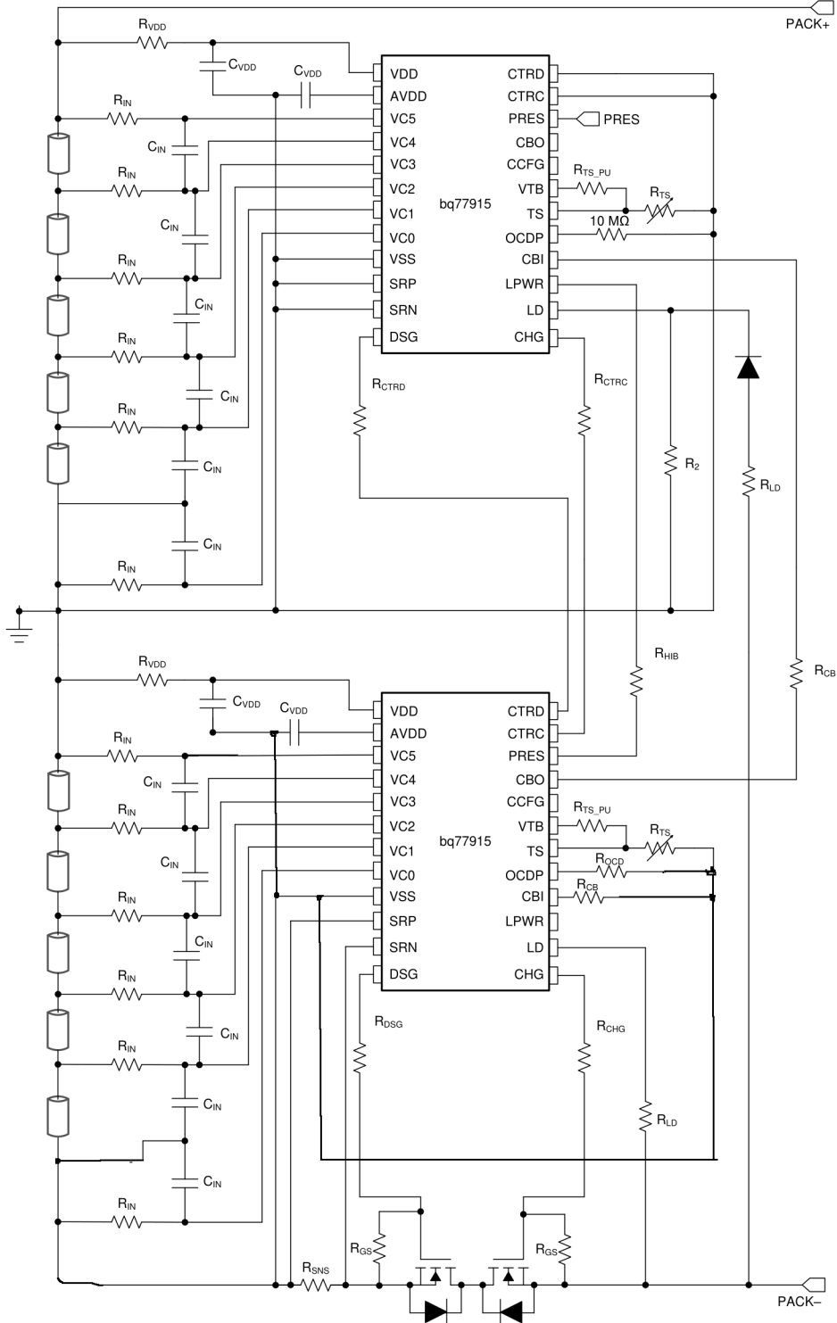
Figure 9-14. 10-Series Configuration with Internal Cell Balancing and HIBERNATE Mode Enabled
