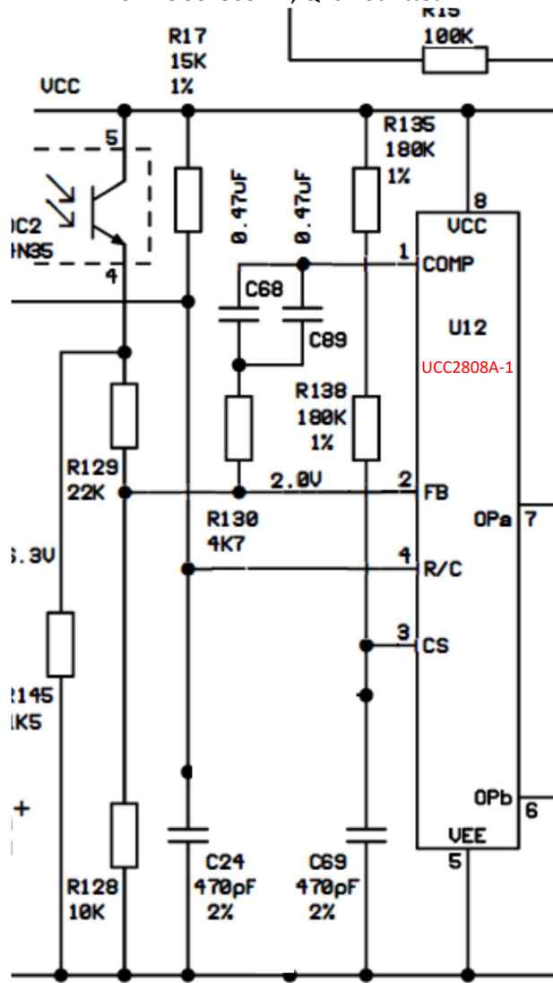
VARIANT: U12 UCC2808A-1, Q40 not fitted
