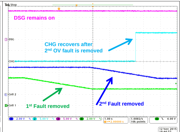
Figure 29. OV Fault Recovery
