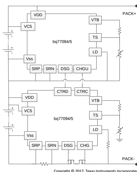
Simplified Schematic
