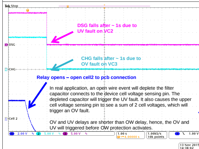
Figure 32. OW Fault Protection - Open Cell2 To PCB Connection
