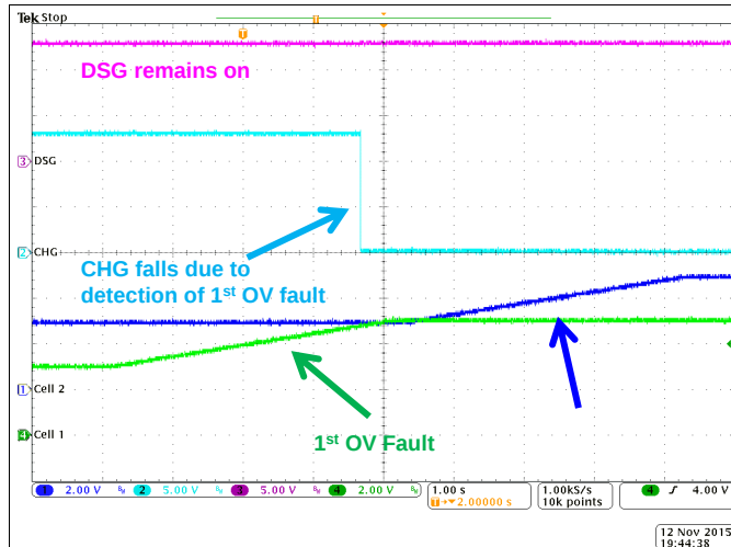
Figure 28. OV Fault Protection
