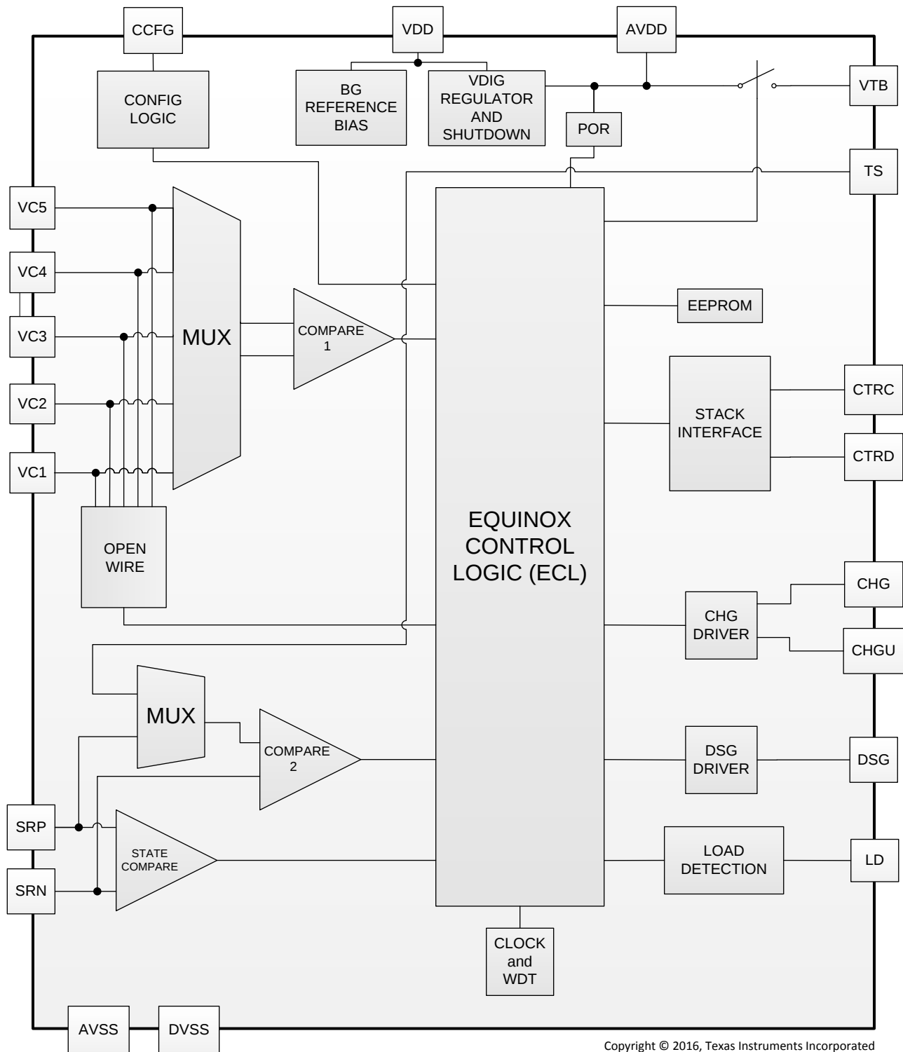
Figure 8. bq77904 and bq77905 Block Diagram
