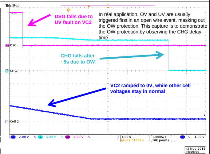
Figure 33. OW Fault Protection - Ramping Down Cell2 Voltage
