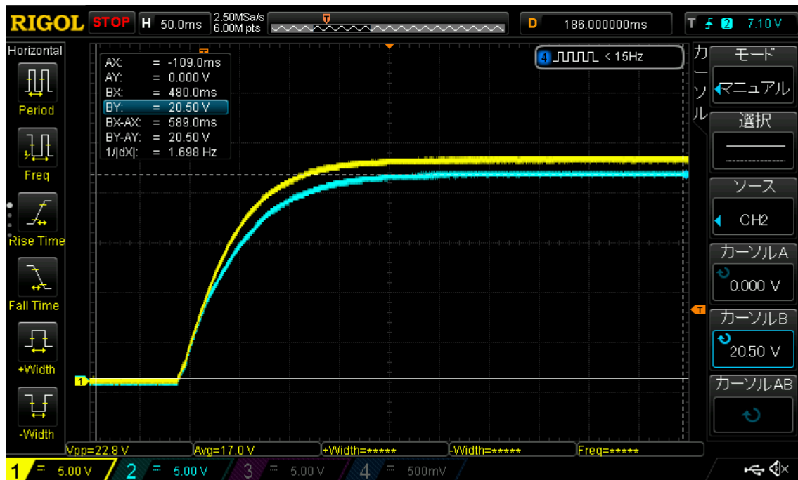
Fig4. Startup waveform (Yellow: VIN, Blue: VOUT)
