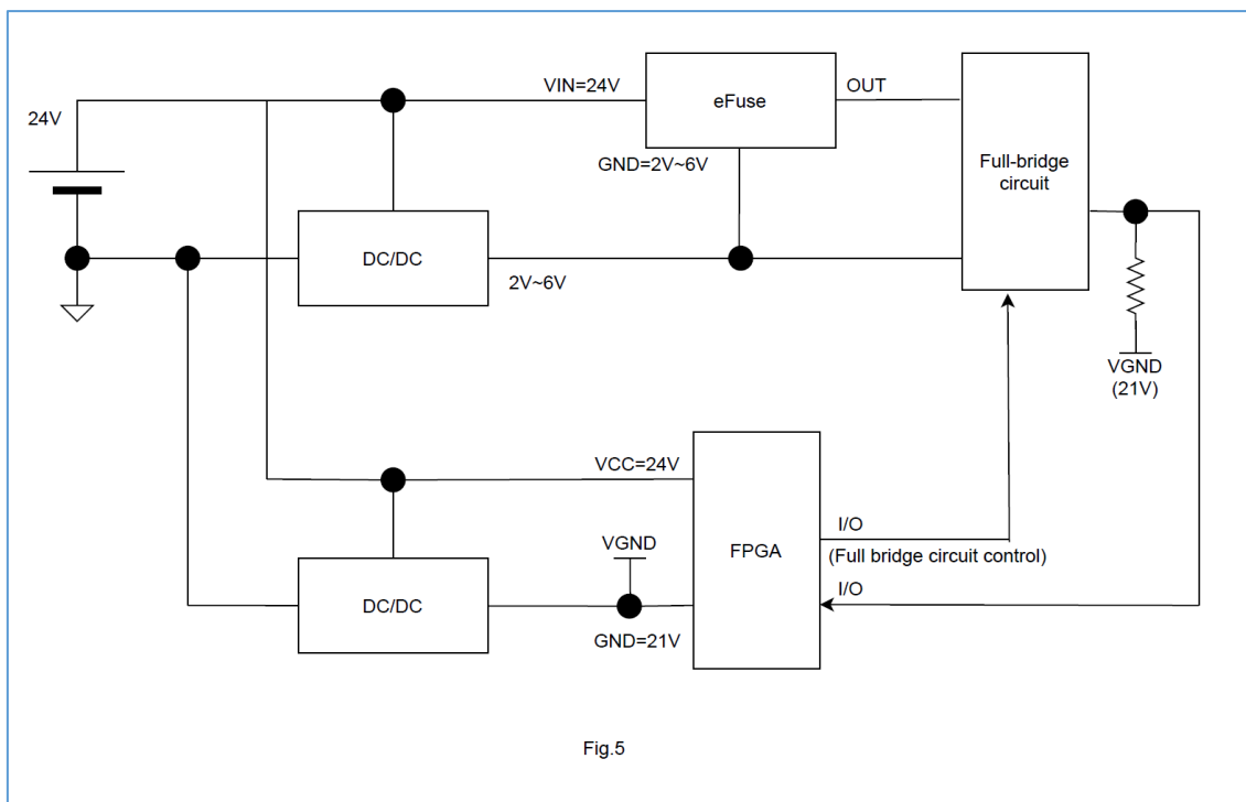
Fig5. Block Diagram
