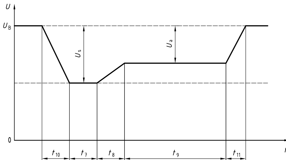
Figure 10 — Test pulse 4
