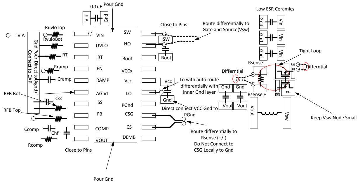
LM5116 Suggested Floorplan
