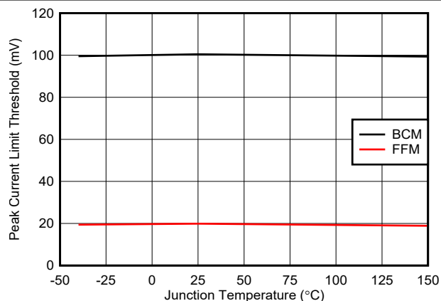
Figure 6-10. Peak Current Limit Thresholds vs. Temperature
