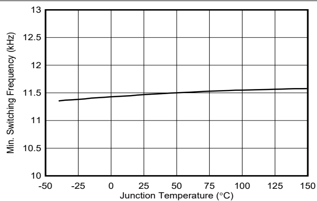
Figure 6-12. Minimum Switching Frequency versus Temperature
