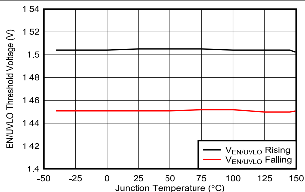
Figure 6-8. EN/UVLO Threshold Voltages versus Temperature
