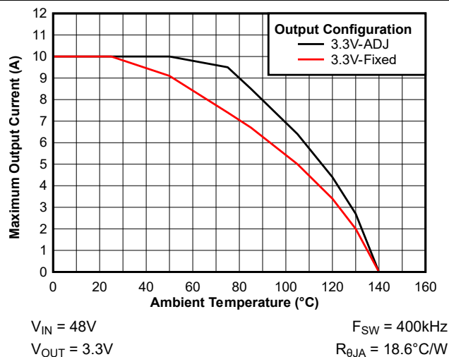
Figure 7-4. Maximum Output Current versus Ambient Temperature
