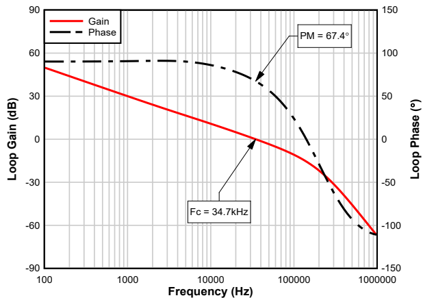
F_C = crossover frequency, PM = phase margin. V_{IN} = 24V F_{SW} = 400kHz FPWM V_{OUT} = 3.3V I_{OUT} = 10A (resistive) L = 2.2μH
