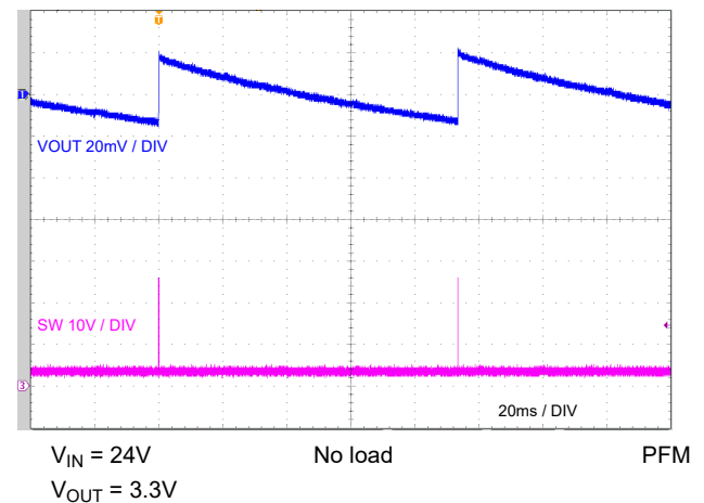
Figure 7-29. PFM Switching
