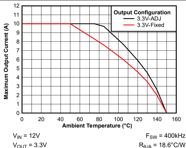
Figure 7-6. Maximum Output Current versus Ambient Temperature
