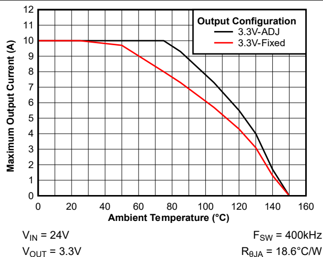
Figure 7-5. Maximum Output Current versus Ambient Temperature
