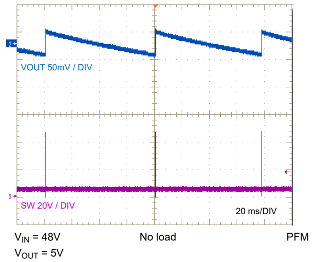
Figure 7-16. PFM Switching
