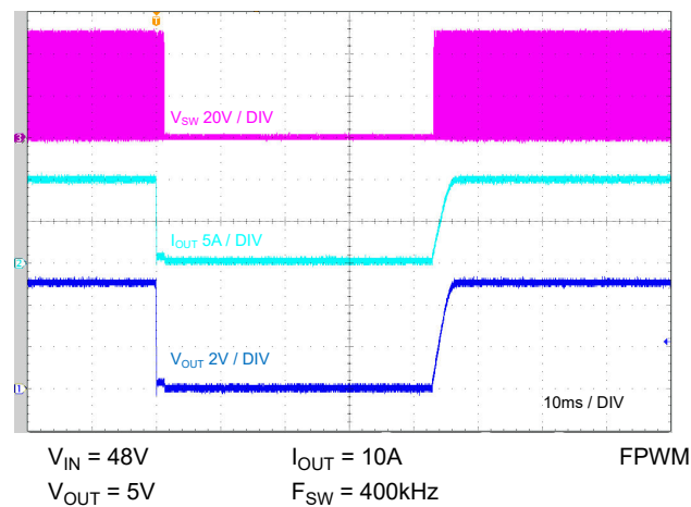
Figure 5-11. Short-Circuit Recovery
