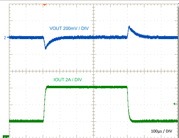
Figure 7-20. Load Transient, 2A to 6A
