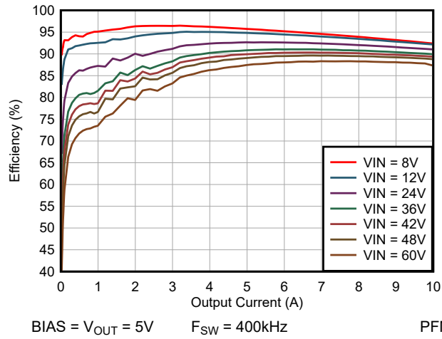
Figure 5-7. Efficiency vs I_{OUT} , Linear Scale
