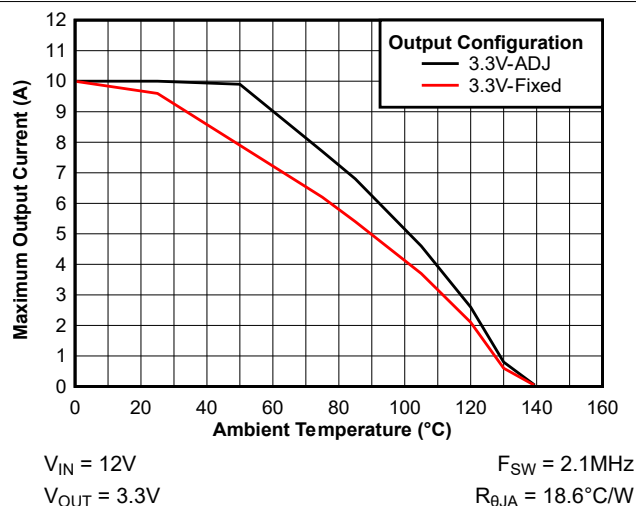
Figure 7-7. Maximum Output Current versus Ambient Temperature
