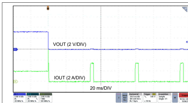
Figure 7-13. Hiccup Entry
