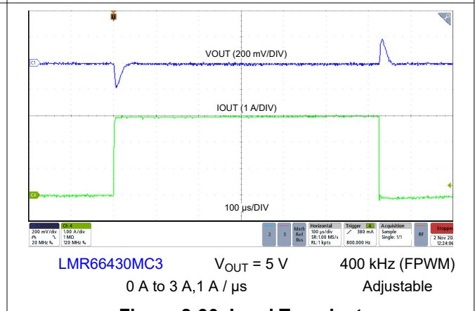
Figure 8-30. Load Transient
