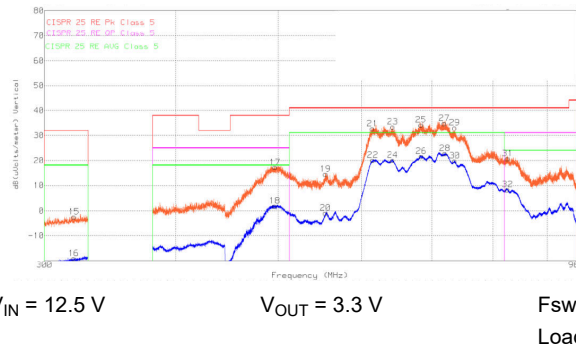
Figure 8-24. CISPR 25 Class 5 Radiated EMI, Log Antenna, Vertical Polarization, 300 MHz - 960 MHz Orange: Peak Detect, Blue: Average Detect
