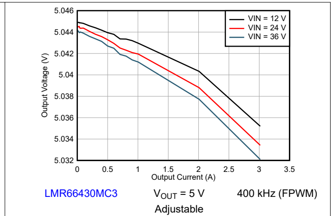
Figure 8-28. Line and Load Regulation
