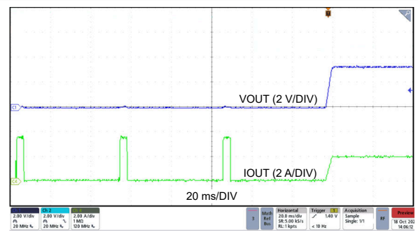
Figure 7-14. Hiccup Exit
