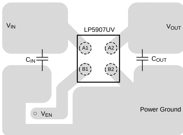
Figure 26. LP5907UV-x.x (DSBGA) Typical Layout
