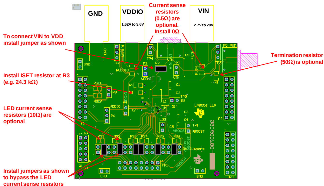
Figure 2: LP8556SQ-EVM Configuration
