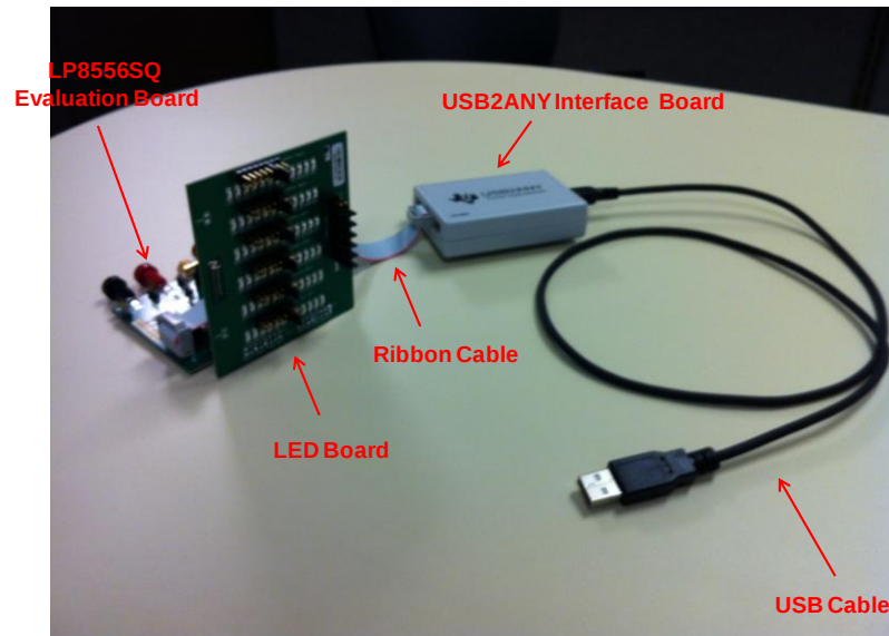
Figure 6: LP8556SQ-EVM Test Setup for Evaluation with Software
