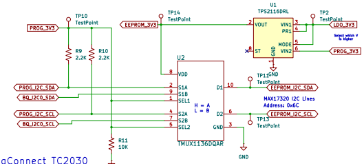
TagConnect TC2030 Programmer
