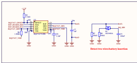
Fuel Gauge (BQ27427)
