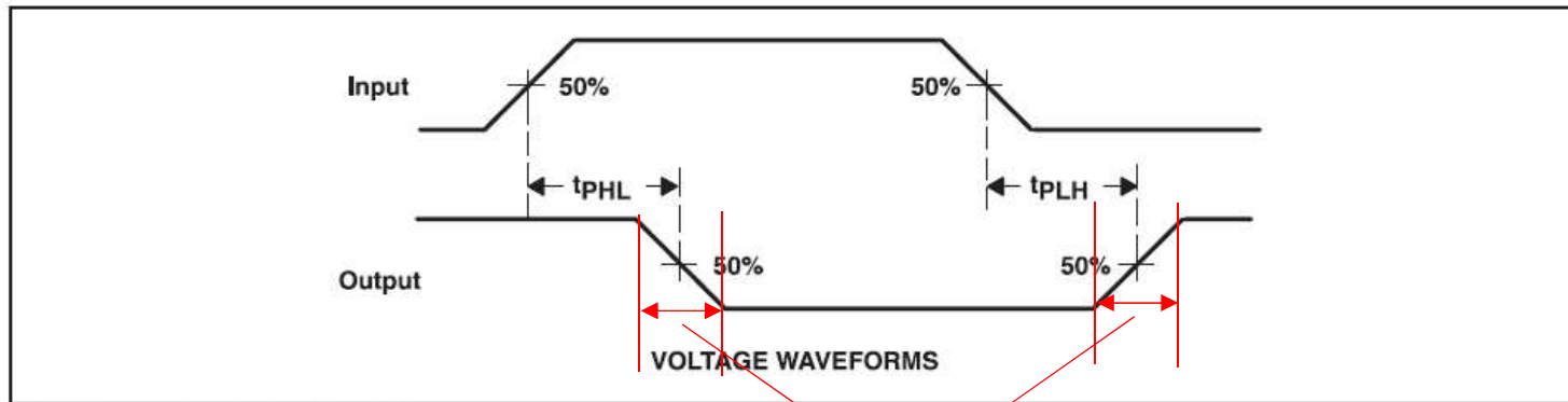
図 9. Propagation Delay-Time Waveforms
