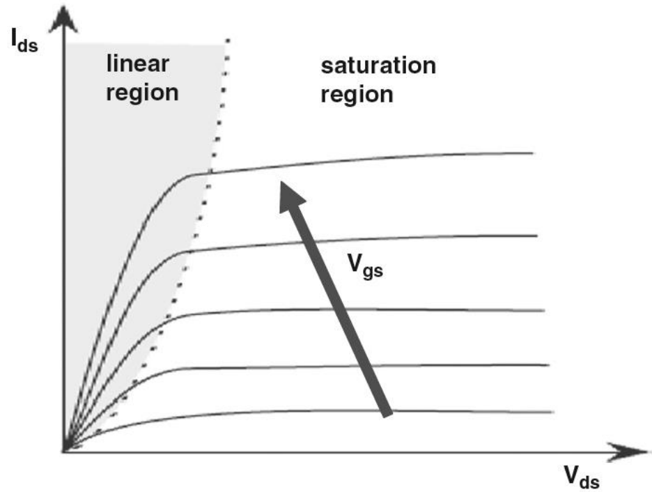
Fig. 1.4 Output I_{ds} - V_{ds} characteristics showing linear and saturation mode
