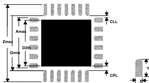
Figure 4. PCB Land Pattern
