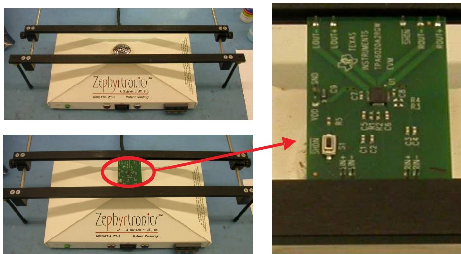
Figure 17. Pre-Heater
