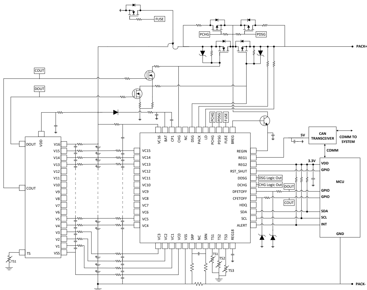
Figure 10-4. BQ77207 with BQ76952
