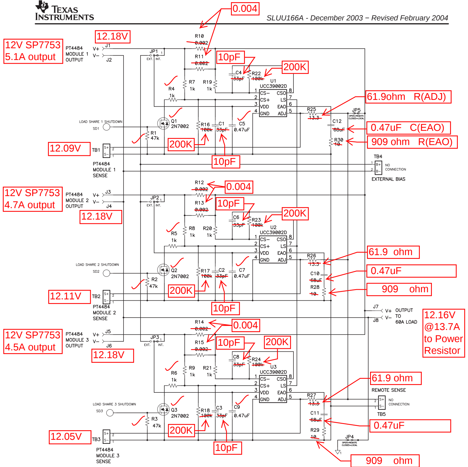
Figure 14. Schematic of Three Paralleled PT4484 Modules
