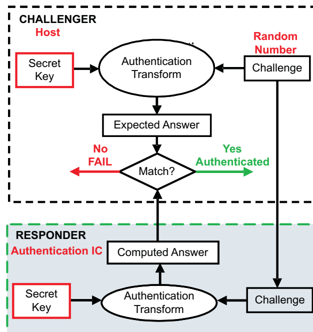
Figure 8. Authentication Scheme for bq26100 or bq27541 (SHA-1/HMAC)
