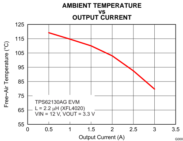
Figure 36. Maximum Ambient Temperature ( f_{SW} = 2.5\text{MHz} )
