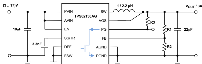
Figure 47. Discharge V_{OUT} Through PG pin
