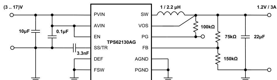
Figure 44. 1.2V/3A Power Supply
