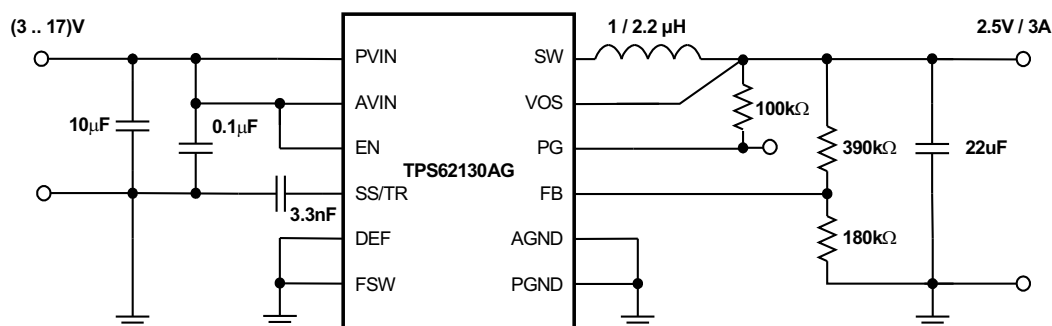
Figure 1. Typical Application
