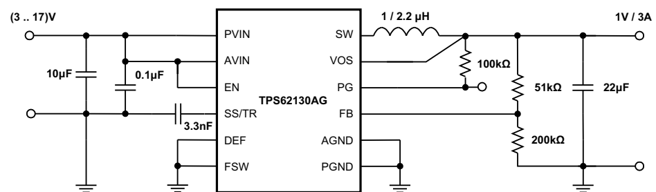
Figure 45. 1V/3A Power Supply
