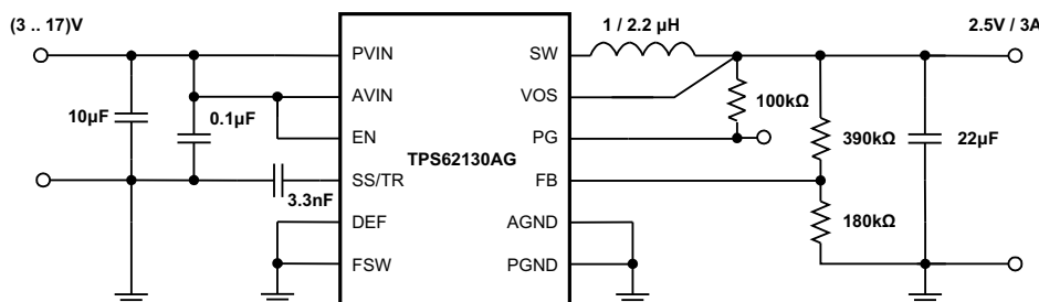
Figure 42. 2.5V/3A Power Supply
