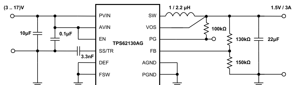
Figure 43. 1.5V/3A Power Supply
