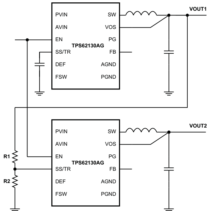
Figure 39. Sequence for Ratiometric and Simultaneous Startup
