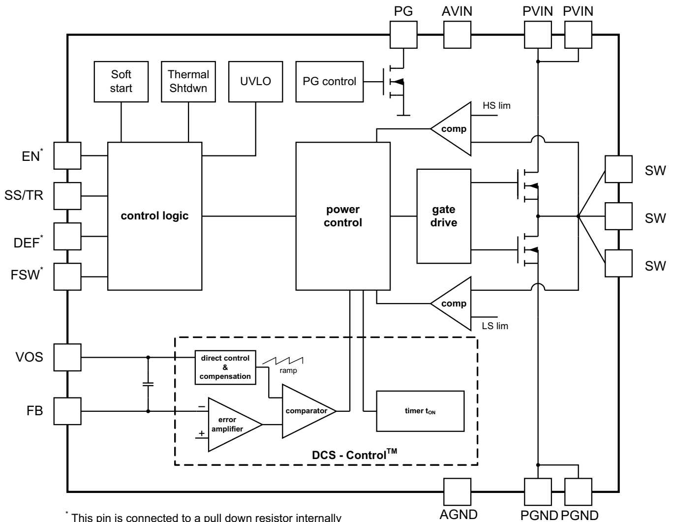
Figure 2. TPS62130AG (adjustable output voltage)
