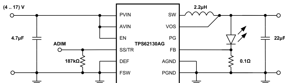
Figure 41. Single Power LED Supply
