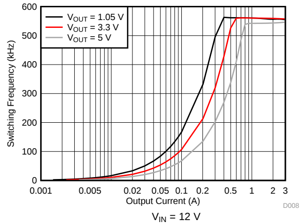
Figure 8. TPS563201 Switching Frequency vs Output Current
