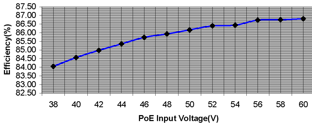
Overall Efficiency vs PoE Vin with 2.1A Load
