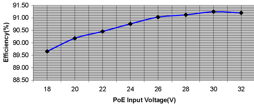
DC/DC Converter Efficiency vs 24Vin with 2.1A Load
