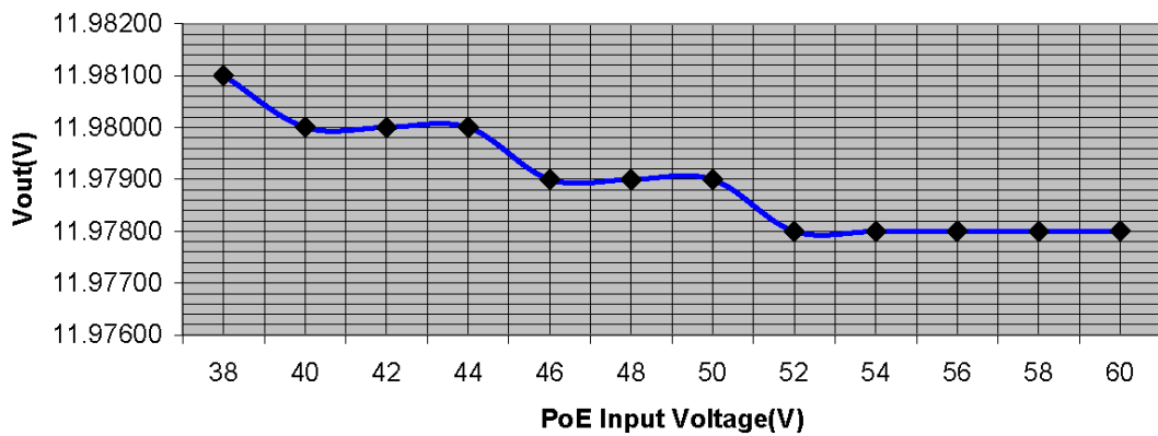
Line Regulation: Vout vs PoE Vin with 2.1A Load
