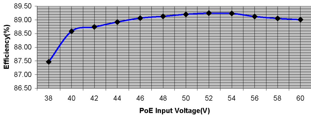
DC/DC Converter Efficiency vs PoE Vin with 2.1A Load
