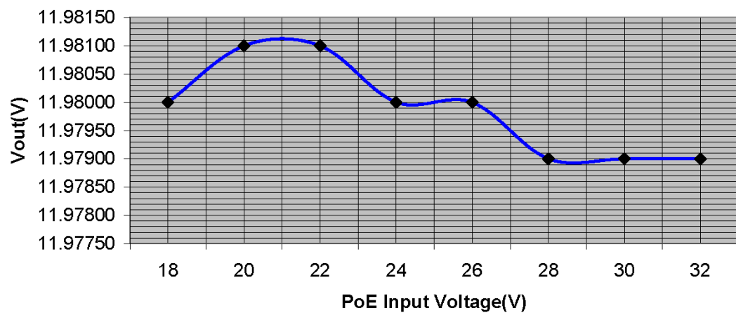
Line Regulation: Vout vs 24Vin with 2.1A Load
