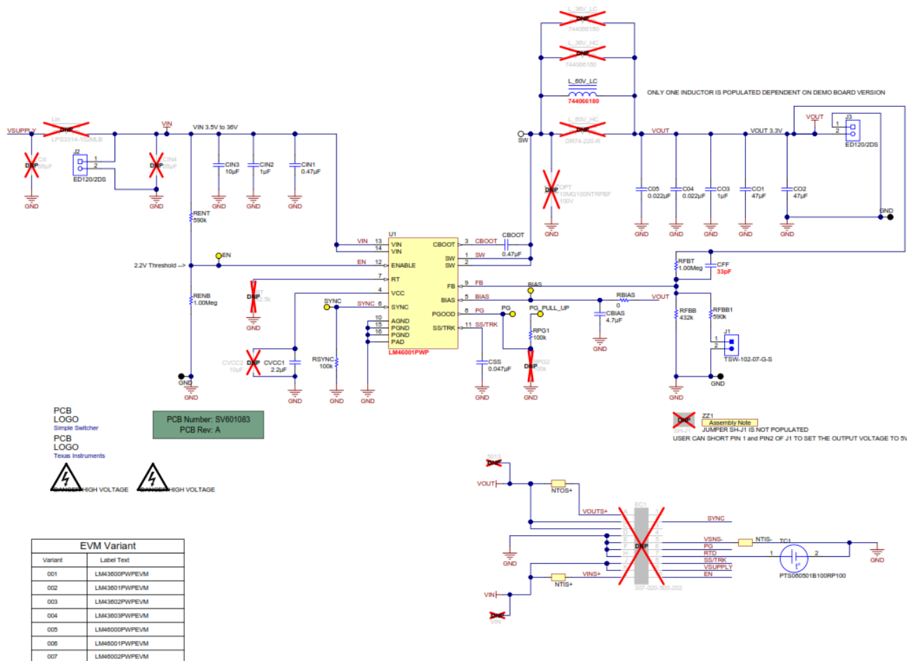
Figure 2. LM46001EVM Schematic
