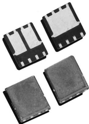
Figure 1. PowerPAK 1212 Devices
