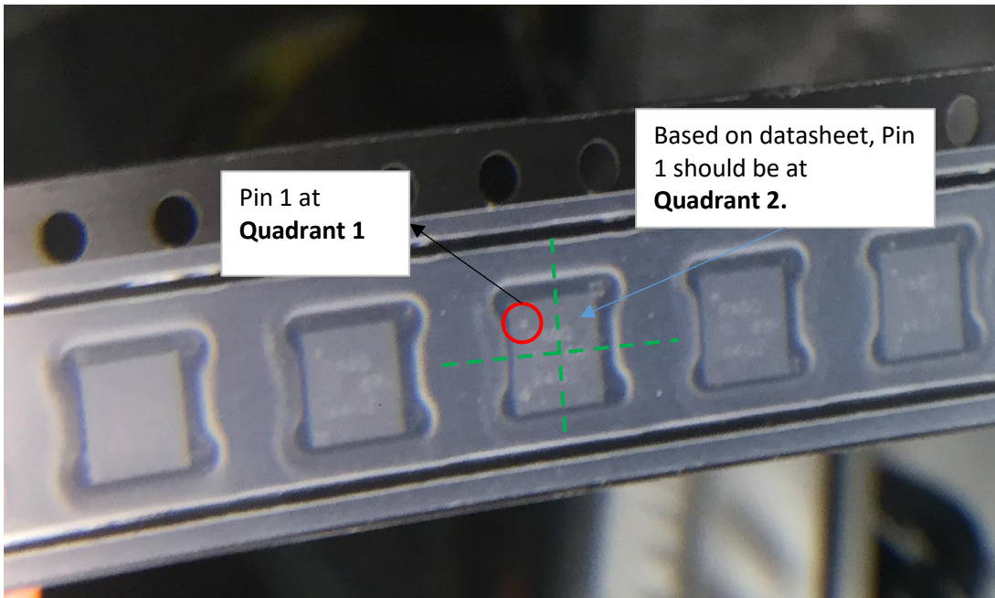
QUADRANT ASSIGNMENTS FOR PIN 1 ORIENTATION IN TAPE
