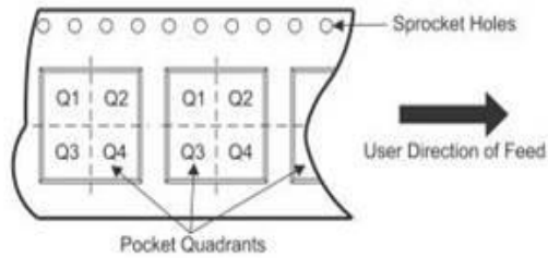
QUADRANT ASSIGNMENTS FOR PIN 1 ORIENTATION IN TAPE
