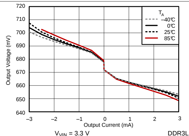
Figure 4. Load Regulation
