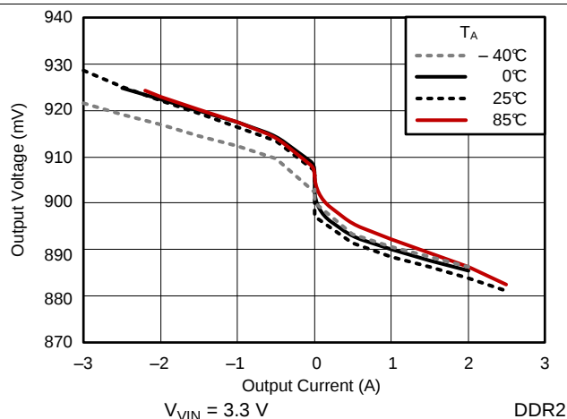
Figure 2. Load Regulation
