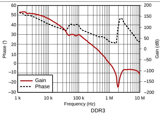
Figure 18. Bode Plot
