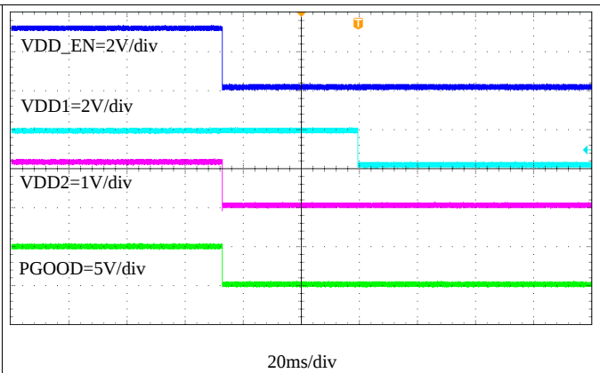
Figure 47. Shutdown Through VDD_EN, I_{VD1OUT} = 1\text{ A} , I_{VD2OUT} = 8\text{ A}
