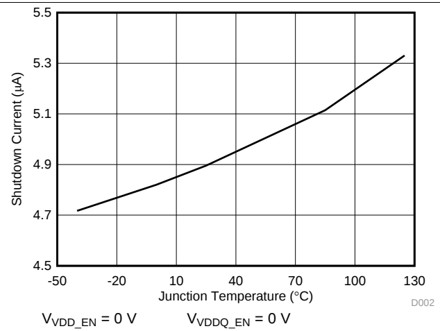
Figure 2. VCC_5V Shutdown Current vs Temperature
