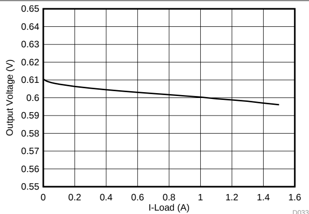
Figure 37. VDDQ Load Regulation, V_{OUT} = 0.6 V
