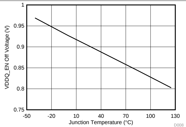
Figure 8. Enable Off Voltage (VDDQ_EN) vs Junction Temperature
