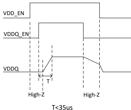
Figure 30. Power Sequence, VDDQ vs VDDQ_EN
