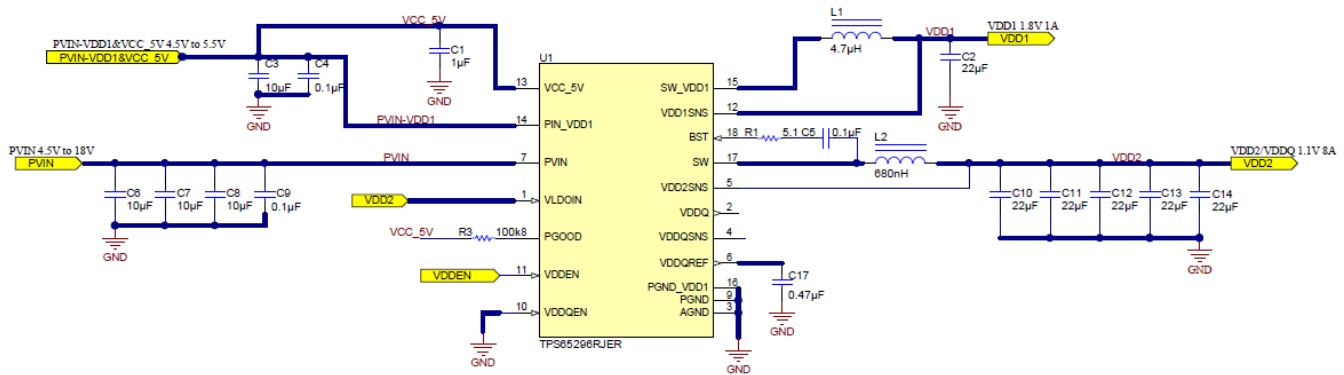
Figure 32. LPDDR4 Application Schematic
