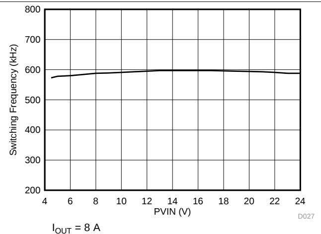
Figure 24. VDD2 Switching Frequency vs Input Voltage
