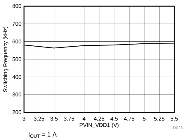
Figure 25. VDD1 Switching Frequency vs Input Voltage
