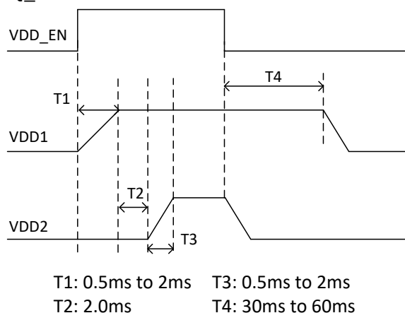
Figure 29. Power Sequence, VDD1 and VDD2 vs VDD_EN
