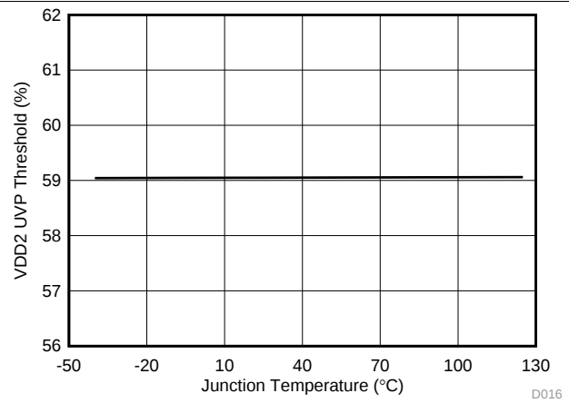
Figure 14. VDD2 UVP Threshold vs Junction Temperature
