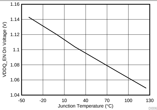
Figure 7. Enable On Voltage (VDDQ_EN) vs Junction Temperature
