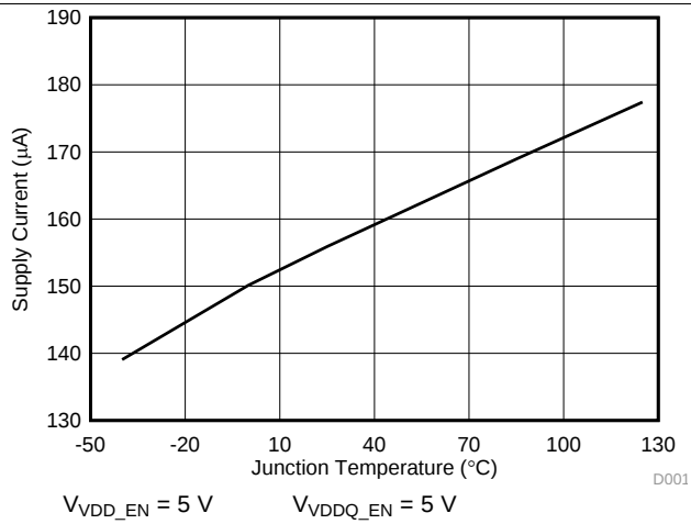
Figure 1. VCC_5V Supply Current vs Junction Temperature
