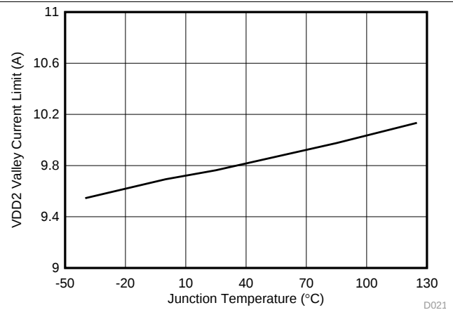
Figure 20. VDD2 Valley Current Limit vs Junction Temperature
