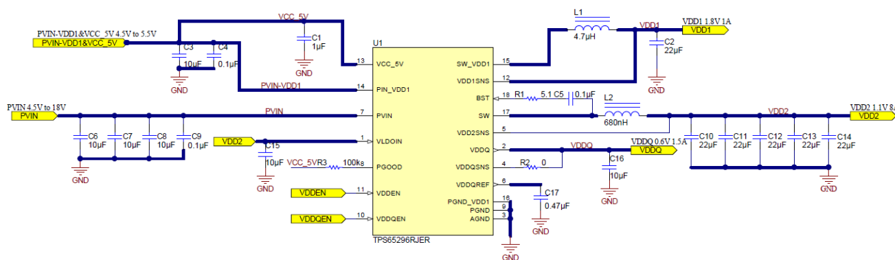
Figure 31. LPDDR4X Application Schematic
