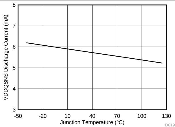
Figure 19. VDDQSNS Discharge Current vs Junction Temperature
