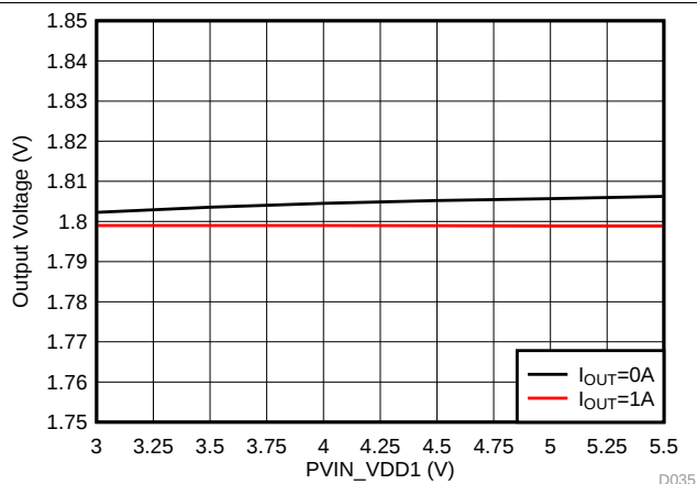
Figure 39. VDD1 Line Regulation, V_{OUT} = 1.8 V
