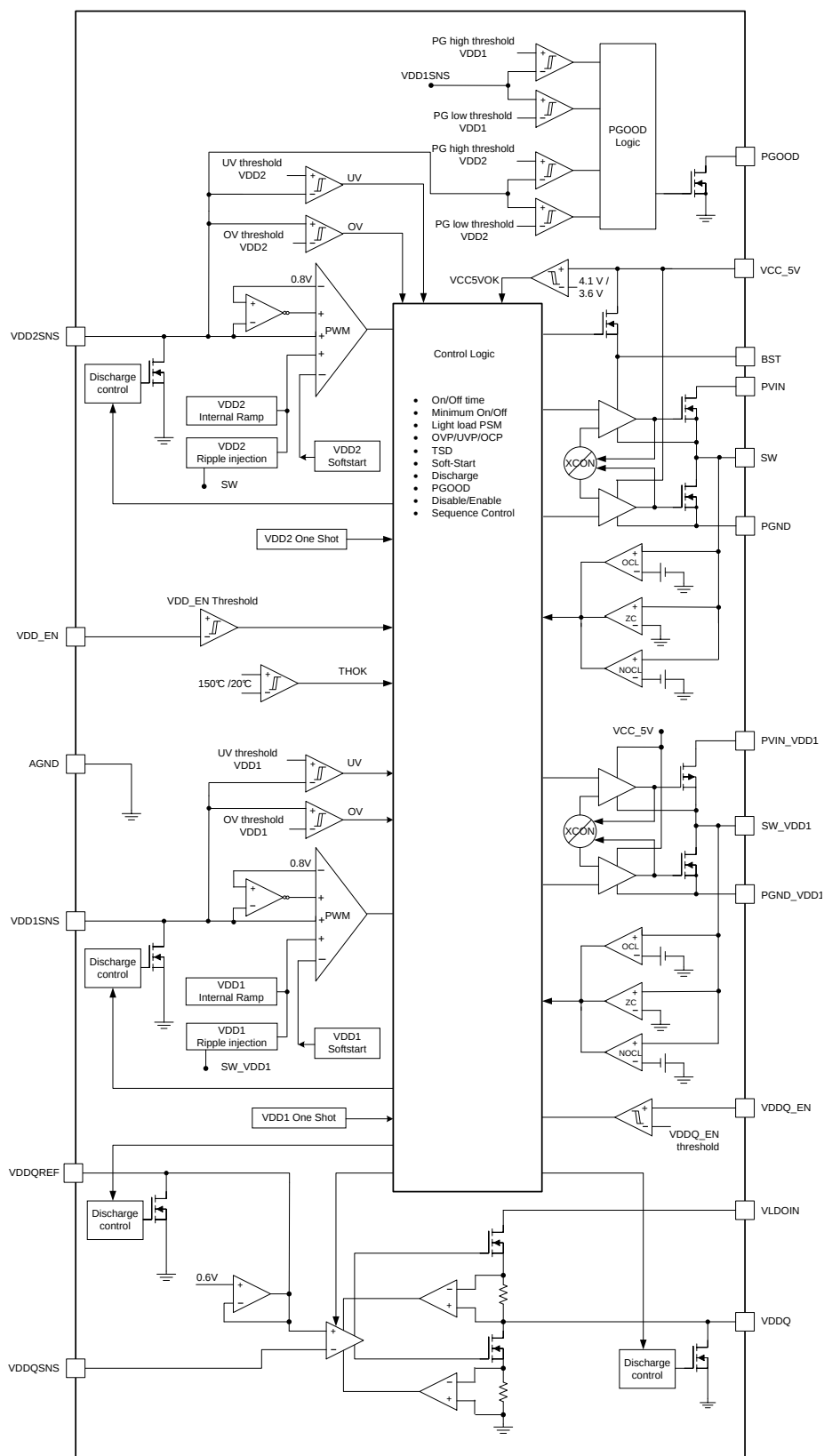
Figure 28. Functional Block Diagram
