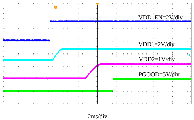
Figure 45. Start-Up Through VDD_EN, I_{VD1OUT} = 1\text{ A} , I_{VD2OUT} = 8\text{ A}
