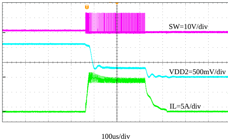
Figure 60. VDD2 Normal Operation to Output Hard Short
