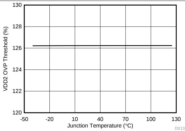
Figure 13. VDD2 OVP Threshold vs Junction Temperature
