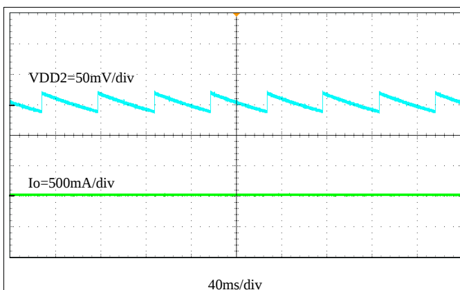
Figure 40. VDD2 Output Voltage Ripple, I_{OUT} = 0 A
