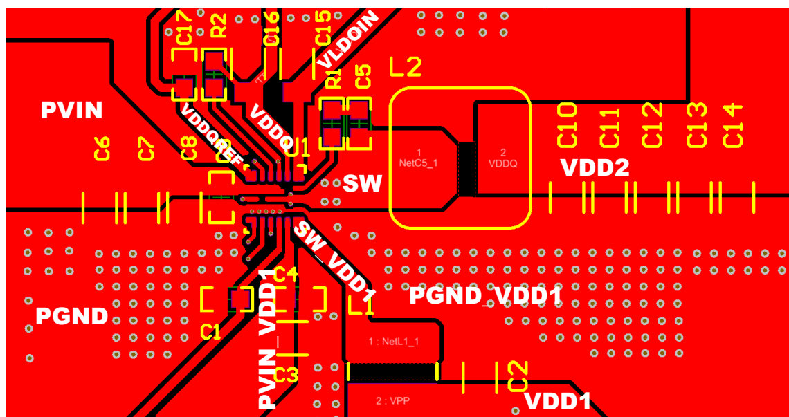
Figure 61. Top-Side Layout
