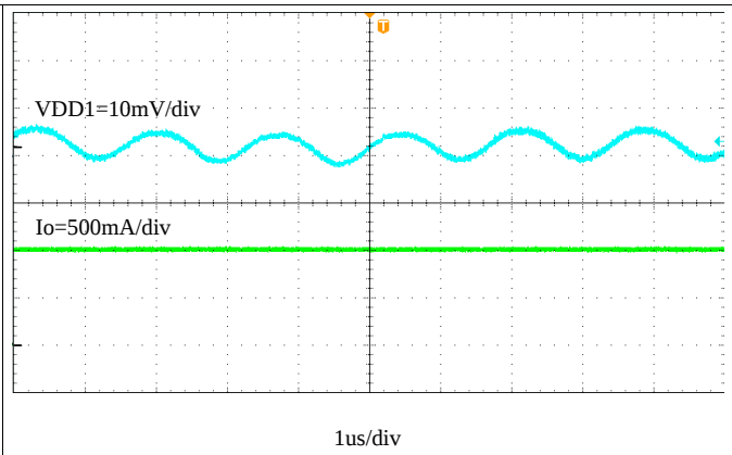
Figure 43. VDD1 Output Voltage Ripple, I_{OUT} = 1\text{ A}
