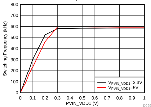
Figure 25. VDD1 Switching Frequency vs Input Voltage
