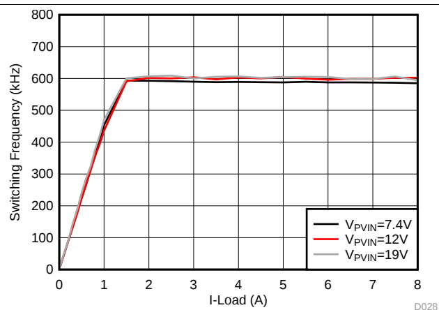
Figure 26. VDD2 Switching Frequency vs Load Current
