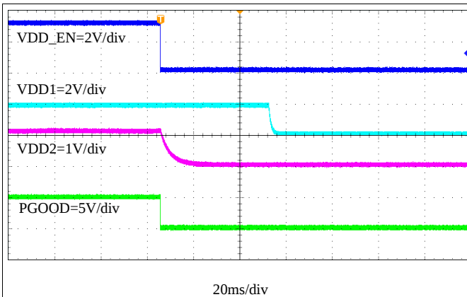
Figure 46. Shutdown Through VDD_EN, I_{VD1OUT} = 0\text{ A} , I_{VD2OUT} = 0\text{ A}
