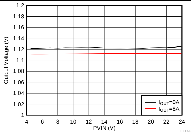
Figure 38. VDD2 Line Regulation, V_{OUT} = 1.1 V
