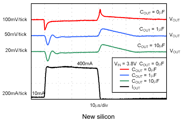
Figure 7-6. TPS73633 Load Transient Response
