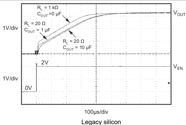
Figure 7-3. TPS73633 Turn-On Response
