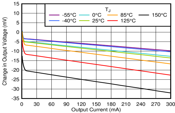
Figure 6-7. Load Regulation vs I_{OUT}
