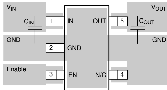
Figure 10-1. DBV Package (SOT-23) Typical Layout
