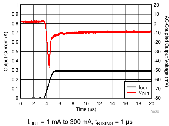
Figure 6-51. Load Transient
