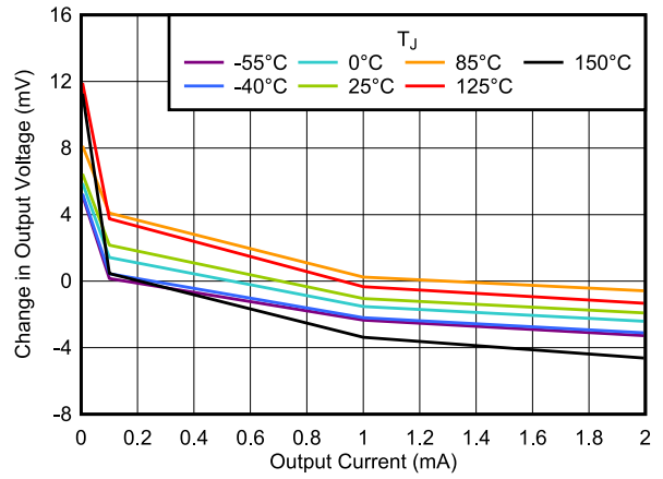
Figure 6-8. Load Regulation vs I_{OUT}
