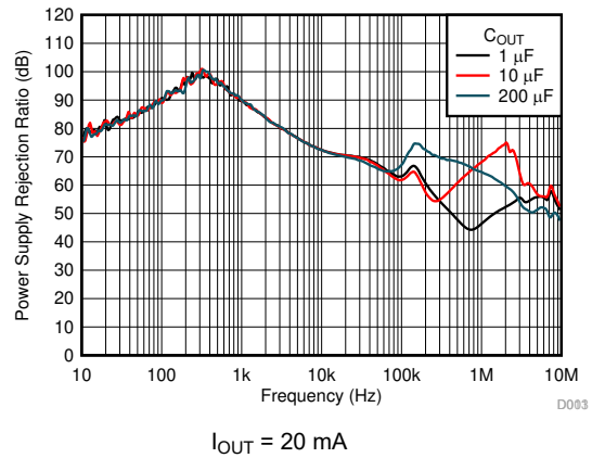
Figure 6-64. PSRR vs Frequency and C_{OUT}
