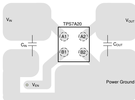
Figure 10-3. YCK Package (DSBGA) Typical Layout
