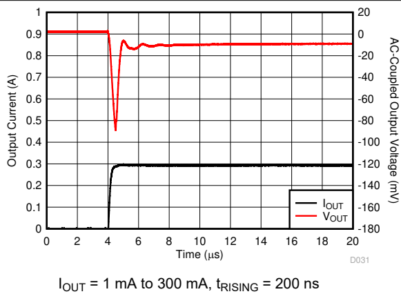
Figure 6-53. Load Transient
