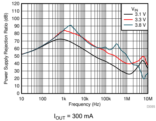
Figure 6-62. PSRR vs Frequency and V_{IN}
