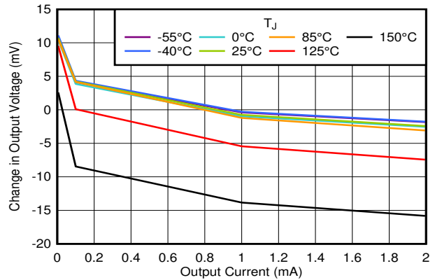
Figure 6-8. Load Regulation vs I_{OUT}
