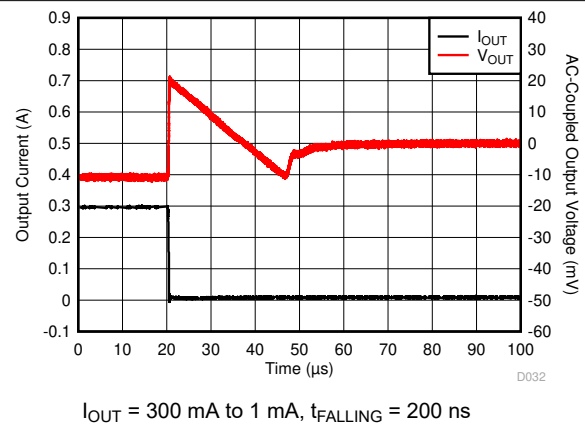
Figure 6-54. Load Transient
