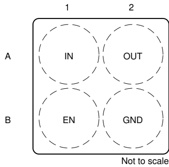
Figure 5-1. YCK Package (Preview), 4-Pin DSBGA, Top View
