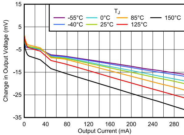
Figure 6-7. Load Regulation vs I_{OUT}
