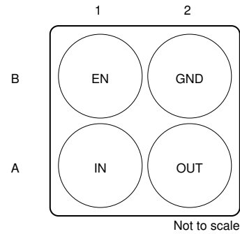
Figure 5-2. YCK Package (Preview), 4-Pin DSBGA, Bottom View
