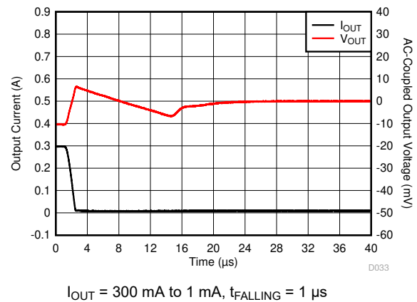
Figure 6-52. Load Transient
