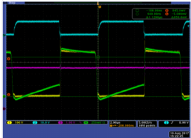
CH1 = V_{DS} CH2 = V_{DR} CH3 = V_{ZC}
