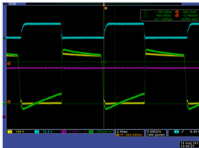
CH1 = V_{DS} CH2 = V_{DR} CH3 = V_{ZC}
