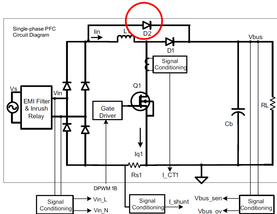
Figure 25. Digitally Controlled Single-Phase PFC System Block Diagram
