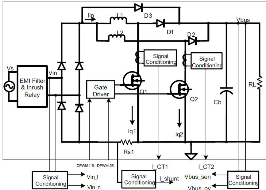
Figure 26. Digitally Controlled 2-Phase PFC System Block Diagram
