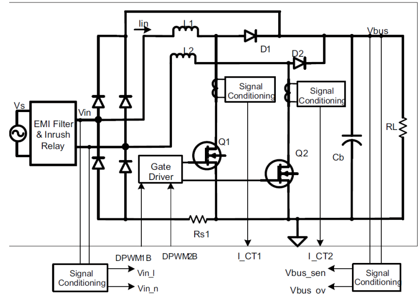
Figure 27. Digitally Controlled Bridgeless PFC System Block Diagram
